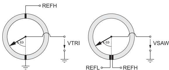
Figure 8: Potentiometer equivalents for resistor mode operations
