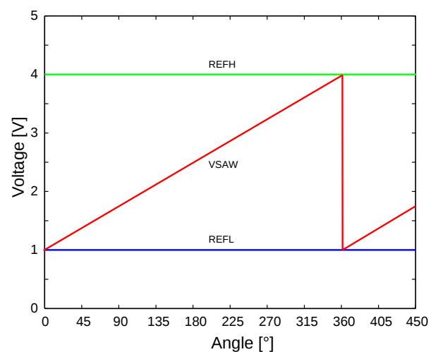
Figure 9: R-Sensor mode with sawtooth output voltage VSAW
