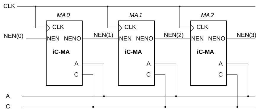
Figure 11: Chain modes for iC-MA
