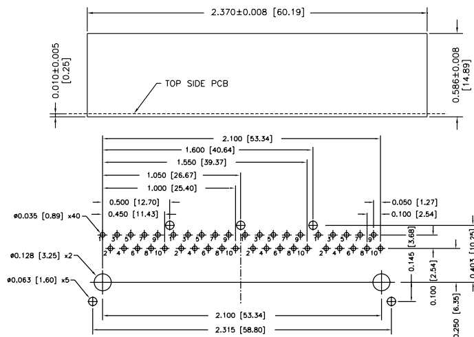
Recommended PC Board Pattern (comp. side)
