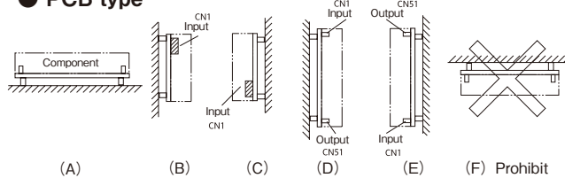
Standard Mounting
