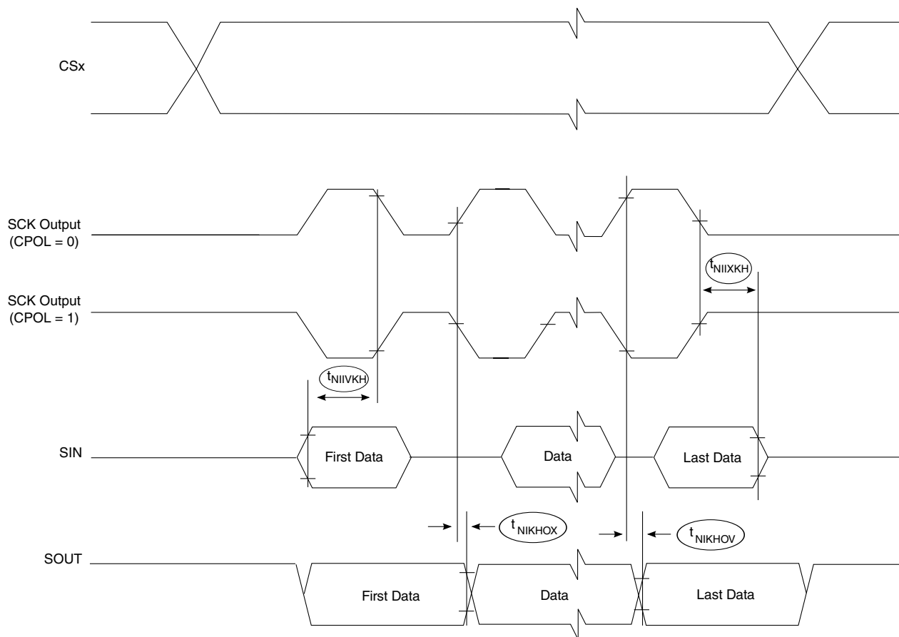
Figure 14. SPI classic SPI timing master, \text{CPHA} = 1
