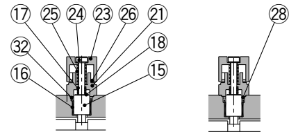
Manual release (Lock type)
