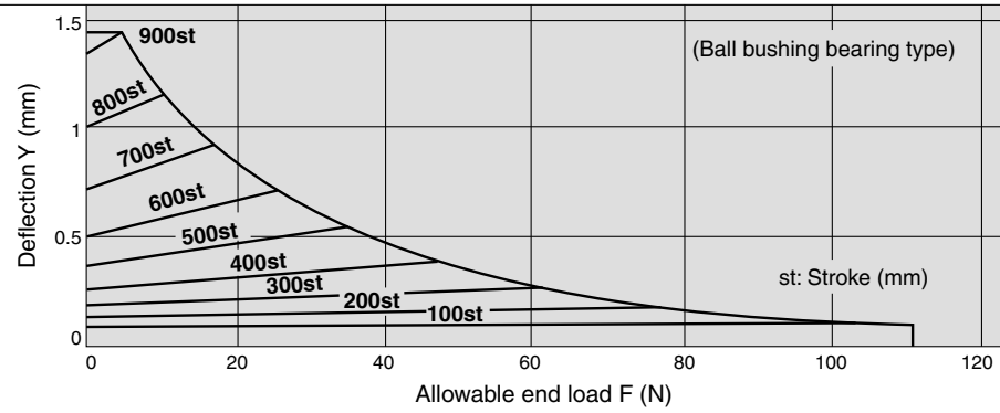
MGGL 50-Stroke
