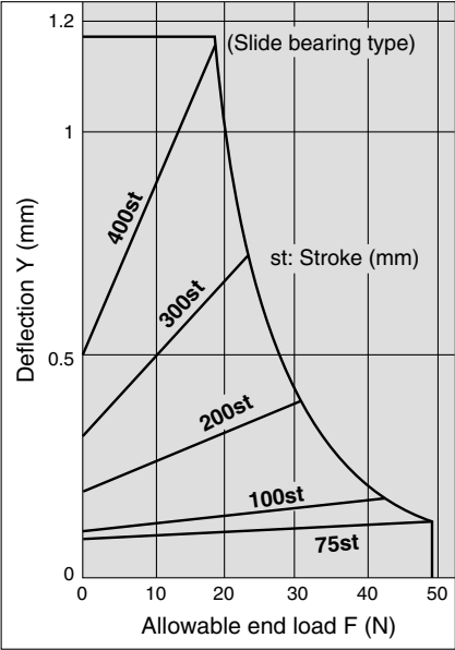
MGGM 20-Stroke
