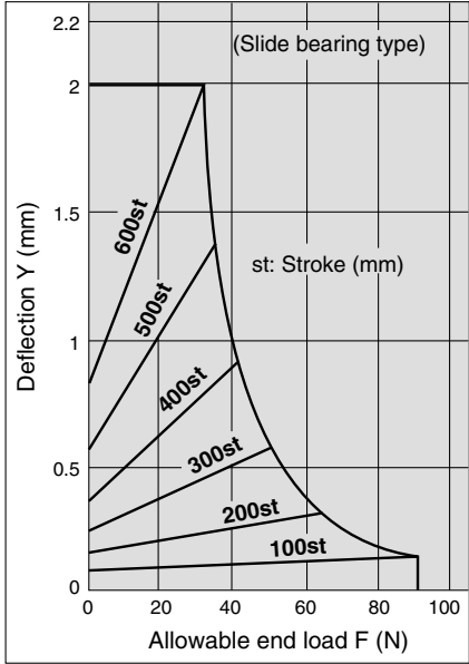
MGGM 32-Stroke
