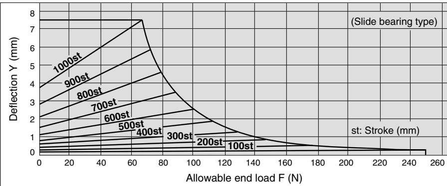
MGGM 50-Stroke
