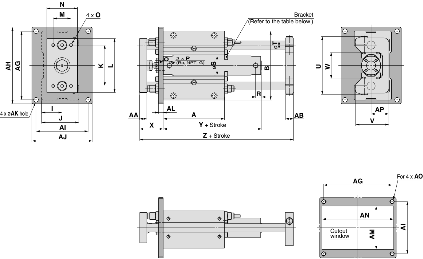
Mounting dimensions
