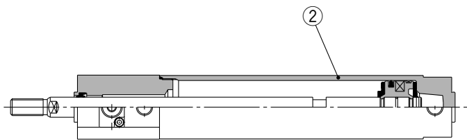
Rod end lock (Base cylinder only)
