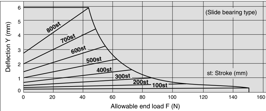
MGGM 40-Stroke
