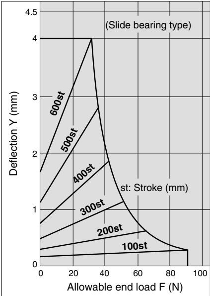
MGGM 32-Stroke
