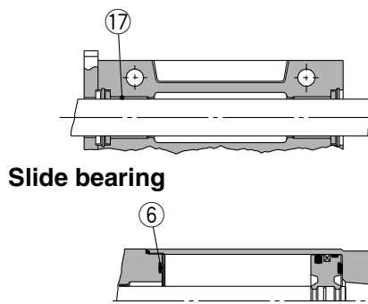
Ball bushing bearing
