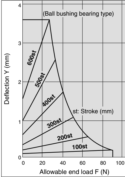
MGGL 32-Stroke
