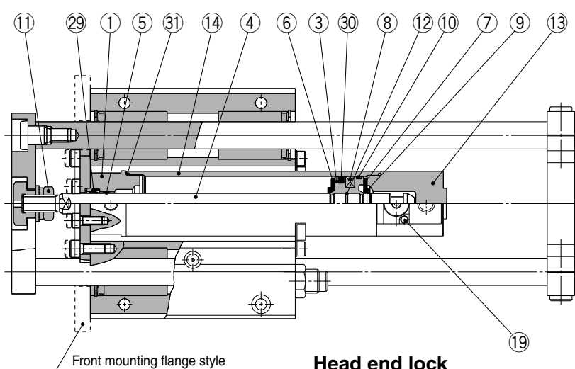
Head end lock
