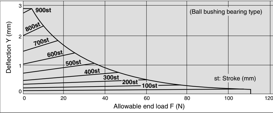
MGGL 50-Stroke
