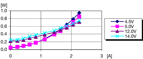
Dissipated power vs. load current and input voltage at T_{ref} = +25^{\circ}\text{C}
