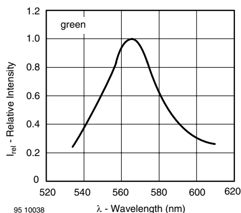
Figure 17. Relative Intensity vs. Wavelength
