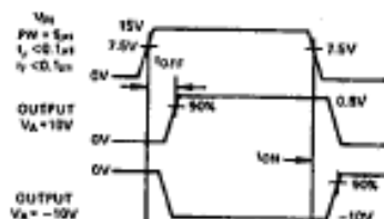
Figure 5: High Level Logic
