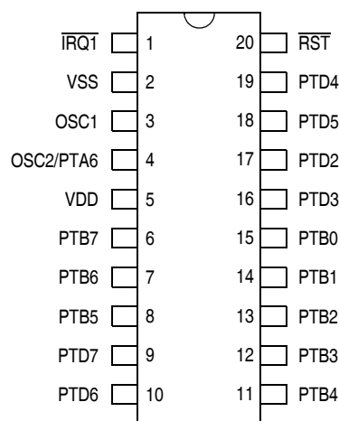
20-PIN ASSIGNMENT MC68H(R)C08JK3/JK1
