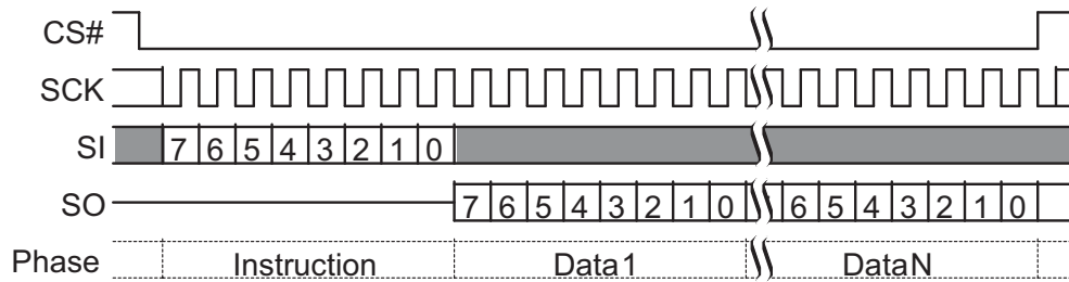
Figure 9.18 AutoBoot Register Read (ABRD 14h) Command
