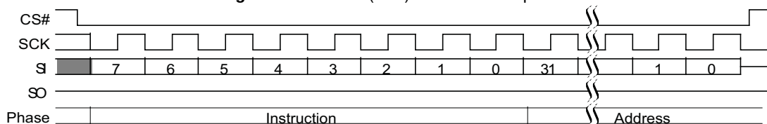
Figure 9.66 PPBP (E3h) Command Sequence
