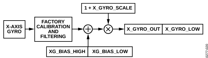
Figure 22. User Calibration Signal Path, Gyroscopes
