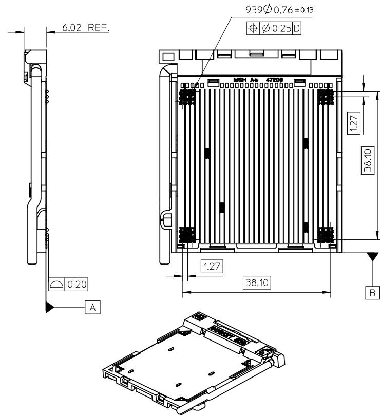
SOCKET 939 CLOSE
