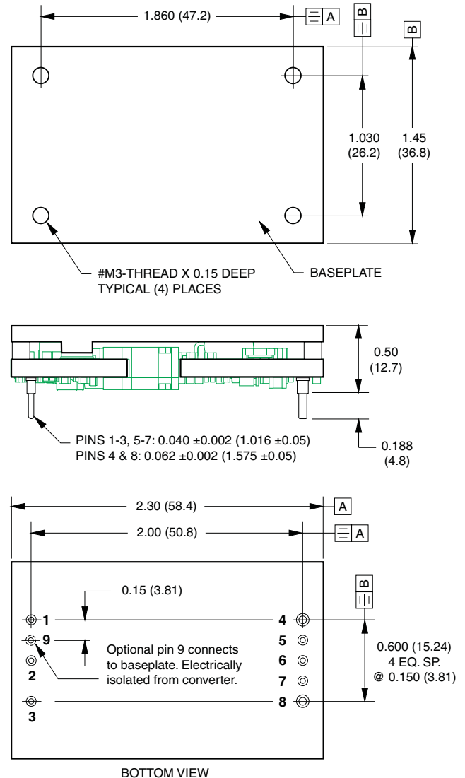
Case C59 with Baseplate
