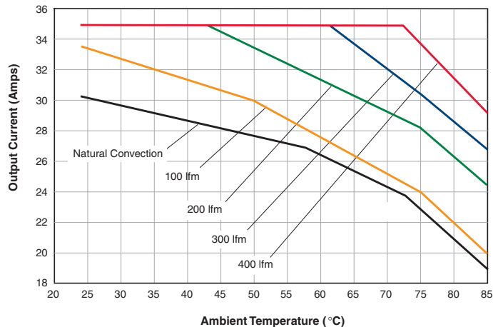
UVQ-3/35-D48 Maximum Current Temperature Derating (With baseplate, V_{IN} = 48V , transverse air flow at sea level)
