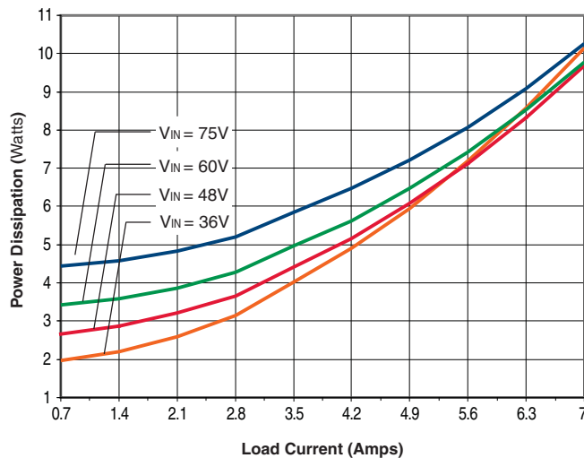
UVQ-15/7-D48N Power Dissipation vs. Load Current @ +25°C
