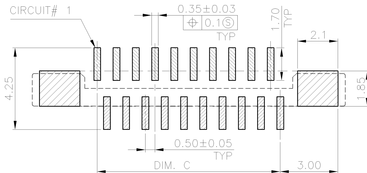
RECOMMENDED PCB LAYOUT (TYPE B)
