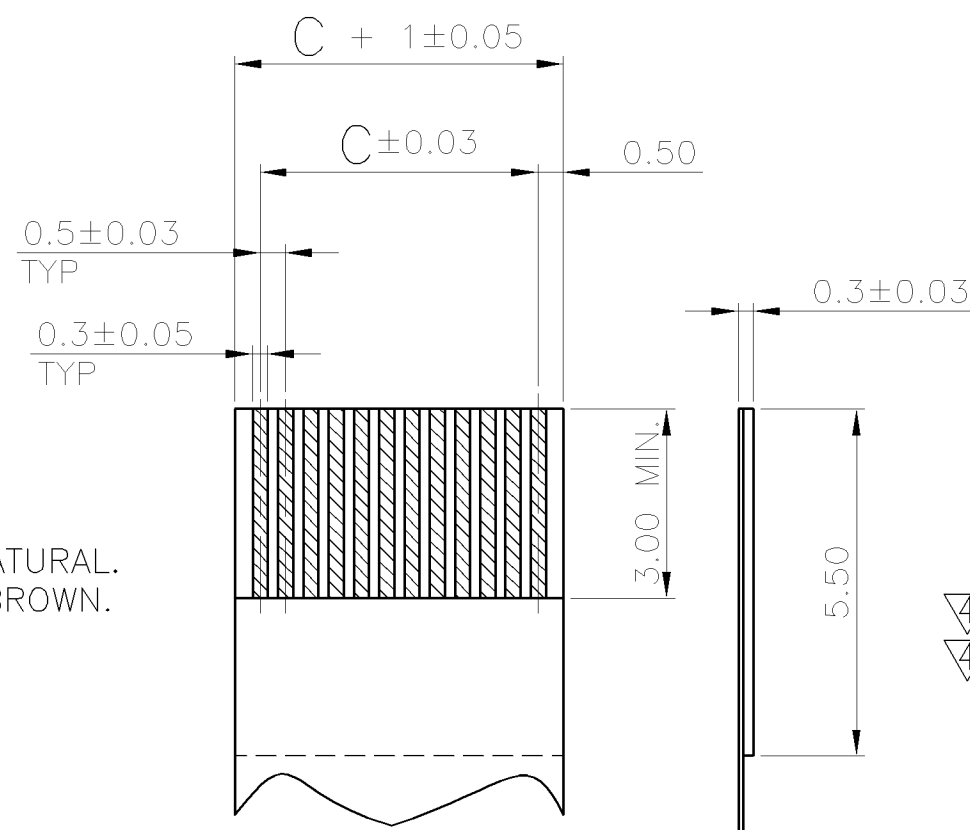
RECOMMENDED FPC/FFC LAYOUT (N = NO. OF CONTACTS)
