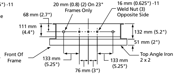
Top Mounting Detail 2.44 m, 2.74 m, 3.51 m (8', 9', 11.5')
