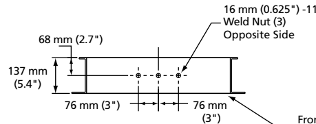
Top Mounting Detail 2.14 m (7')
