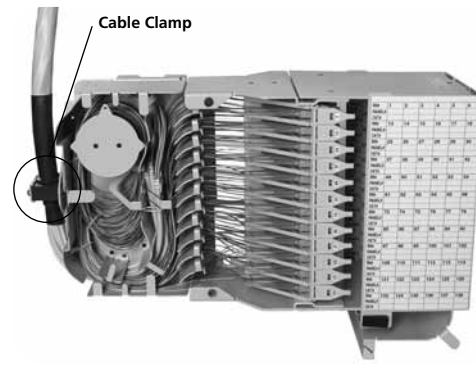
144-Position FTB Loaded with Multifiber Breakout Cable
