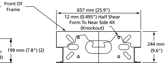
Base Mounting Detail 2.14 m, 2.44 m, 2.74 m, 3.51 m (7', 8', 9', 11.5') (Top View)
