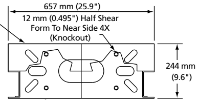
Base Mounting Detail 2.14 m, 2.44 m, 2.74 m, 3.51 m (7', 8', 9', 11.5') (Top View)
