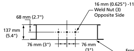
Top Mounting Detail 2.14 m (7')
