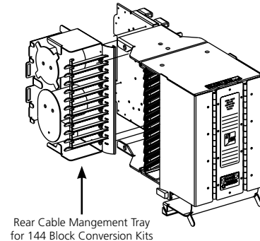
144-Position Right FTB (Shown with IFC Conversion Kit Loaded)
