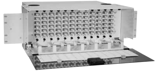
72-Position Termination/Splice Panel
