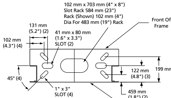
Base Mounting Detail 2.14 m, 2.44 m, 2.74 m, 3.51 m (7', 8', 9', 11.5') (Bottom View)
