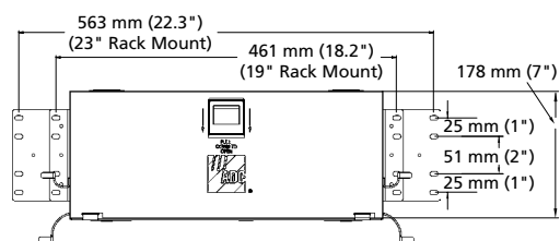
72- or 96-Position Panel (Front View)
