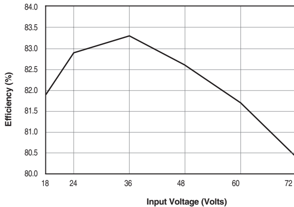
Efficiency vs. Input Voltage (+5V output loaded @ 2.75A, \pm 12V outputs loaded @ \pm 250mA)
