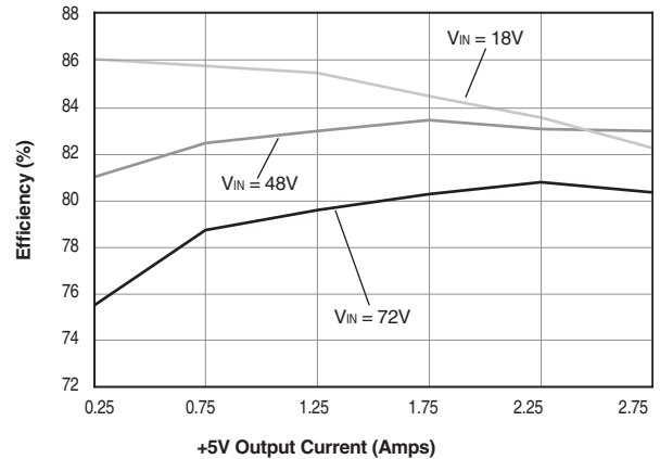
Efficiency vs. +5V Output Loading ( \pm 12V outputs loaded @ \pm 250mA)
