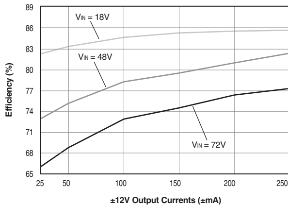
Efficiency vs. \pm 12V Output Loading (+5V output loaded @ 0.55A)
