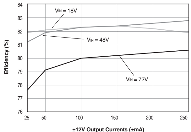
Efficiency vs. \pm 12V Output Loading (+5V output loaded @ 2.75A)
