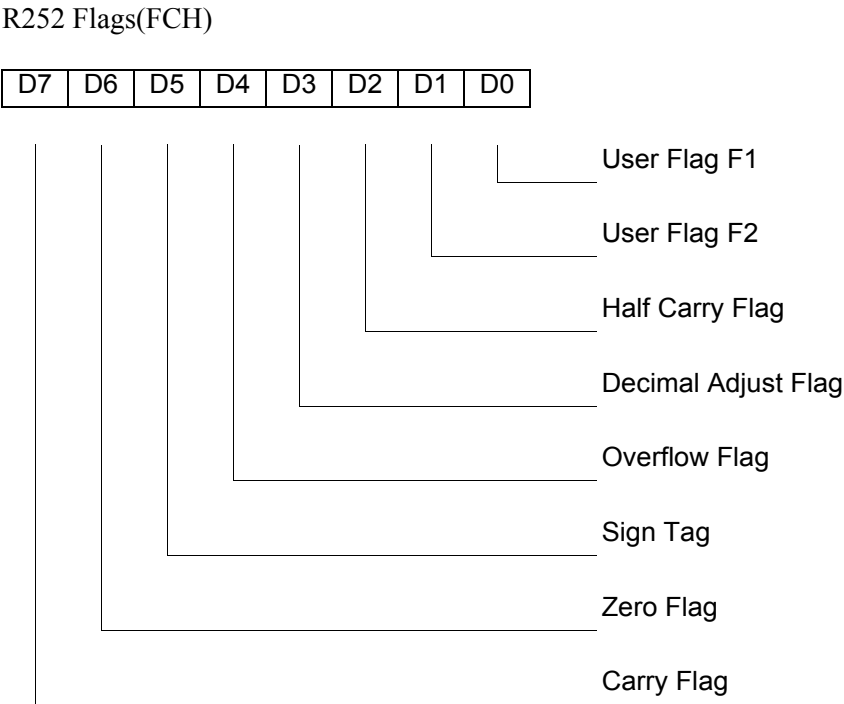
Figure 52. Flag Register (FCH: Read/Write)
