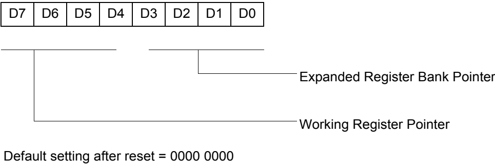
Figure 53. Register Pointer (FDH: Read/Write)
