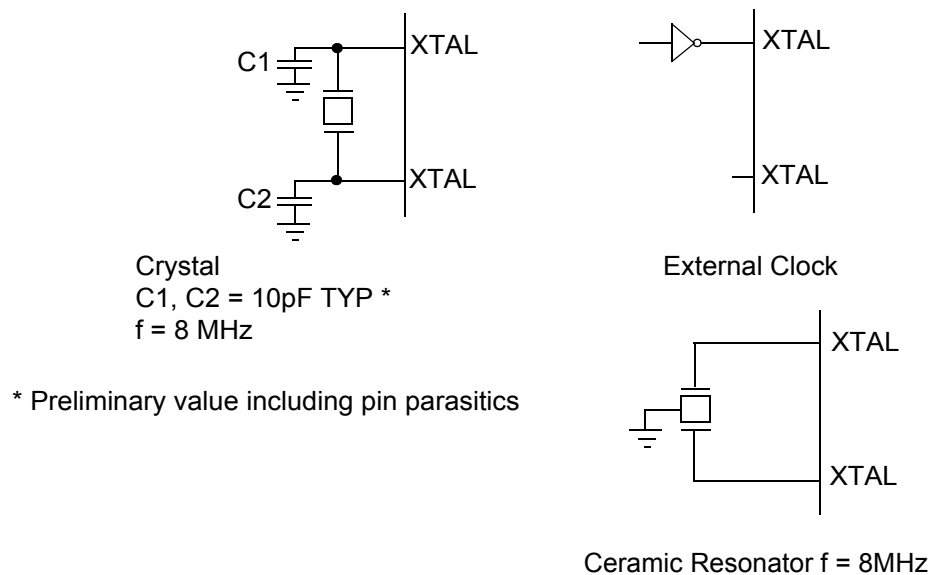
Figure 29. Oscillator Configuration
