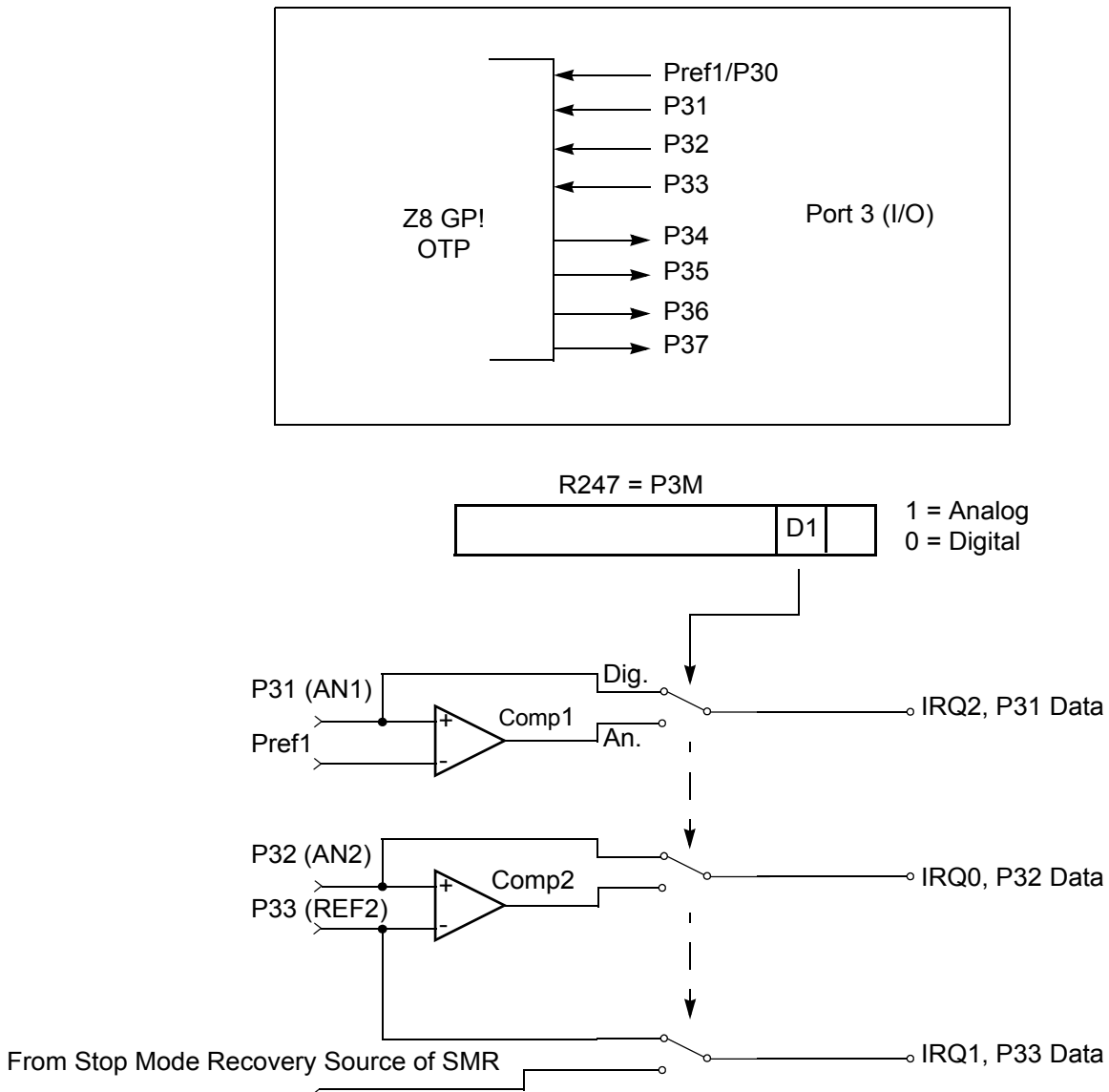
Figure 10. Port 3 Configuration
