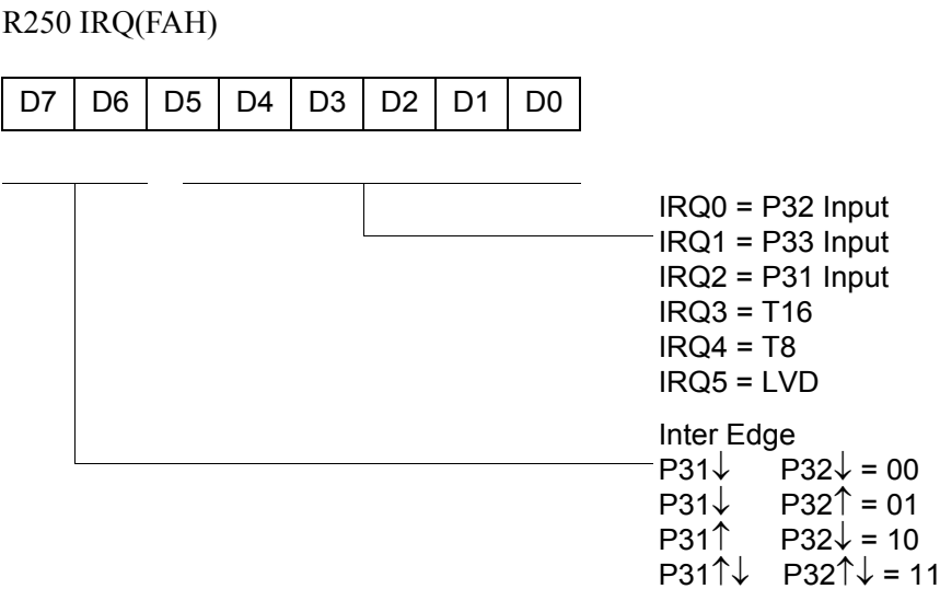
Figure 50. Interrupt Request Register (FAH: Read/Write)
