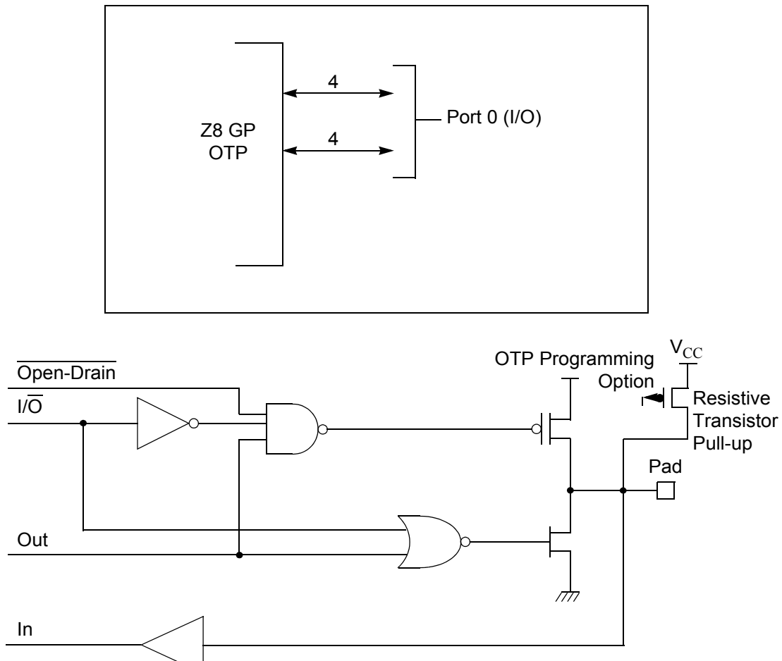
Figure 7. Port 0 Configuration
