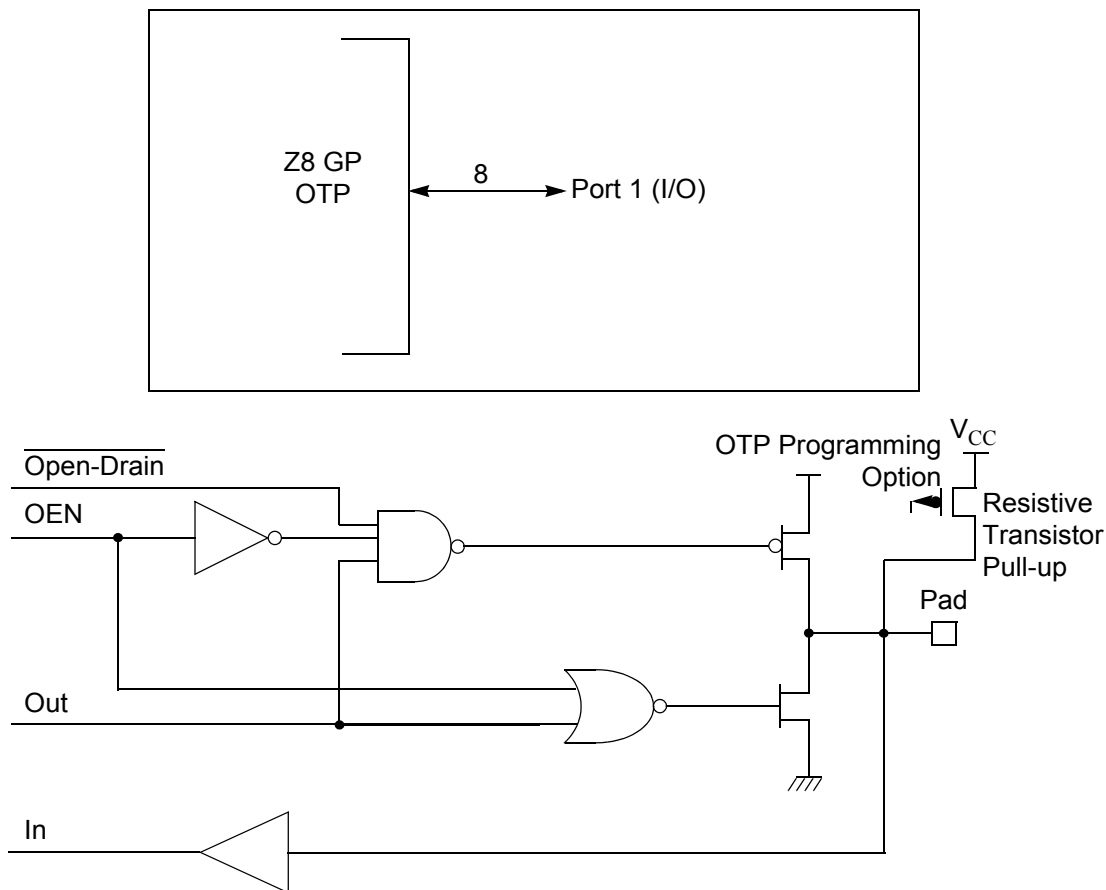
Figure 8. Port 1 Configuration
