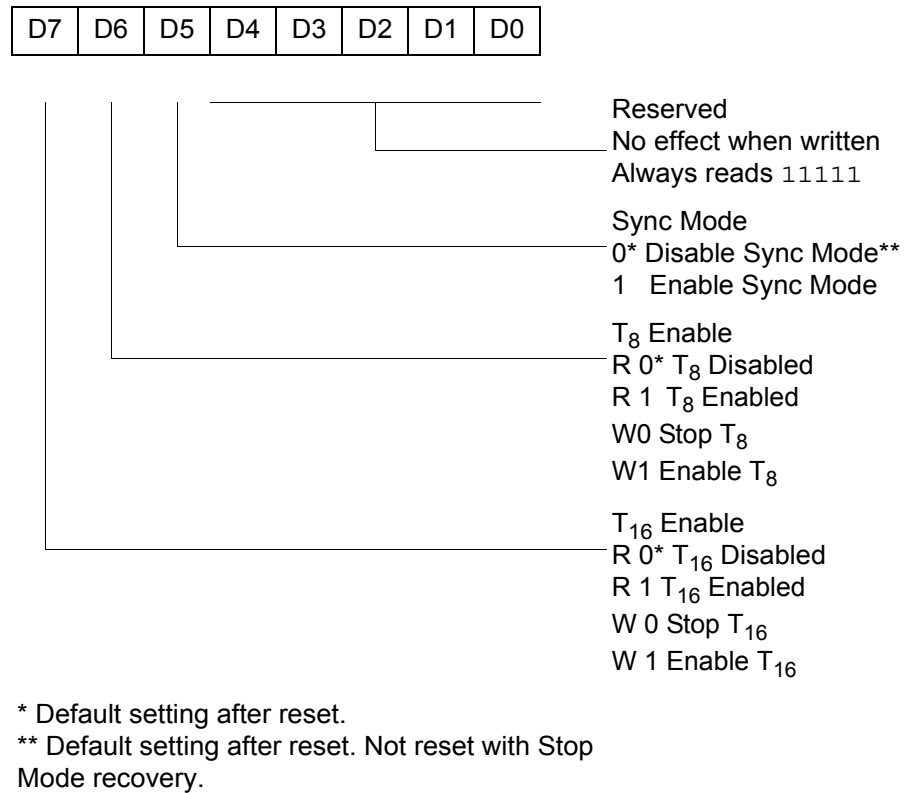
Figure 40. T8/T16 Control Register (0D)03H: Read/Write (Except Where Noted)
