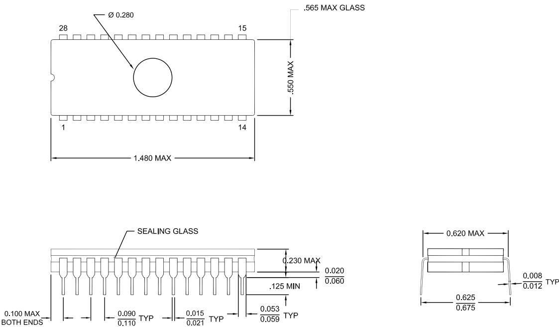
Figure 62. 28-Pin CDIP Package
