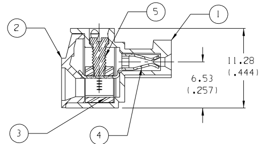
SECTION Z-Z
