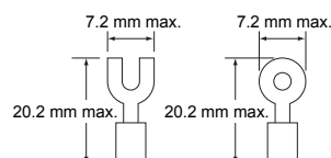
Crimp Terminals with Insulating Sheathes
