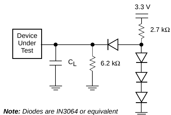
Figure 9. Test Setup
