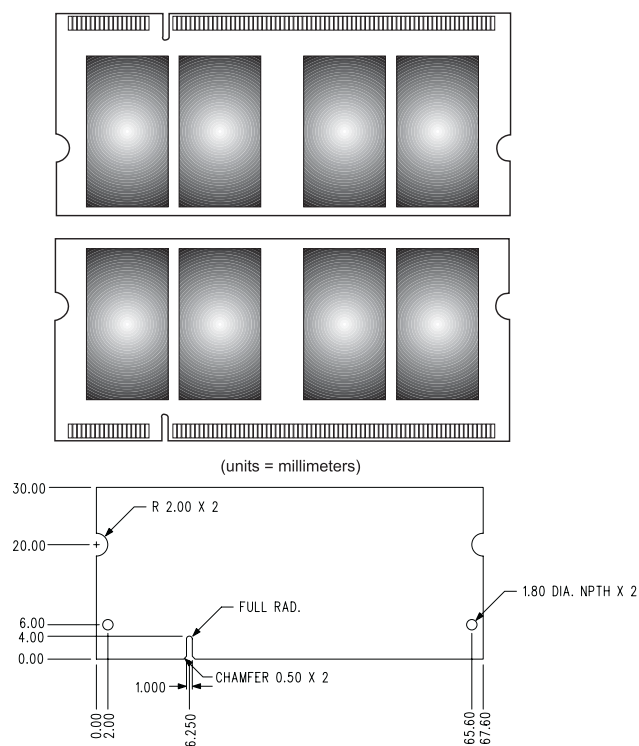
Figure 1: KVR667D2S5/1G 200-Pin SODIMM
