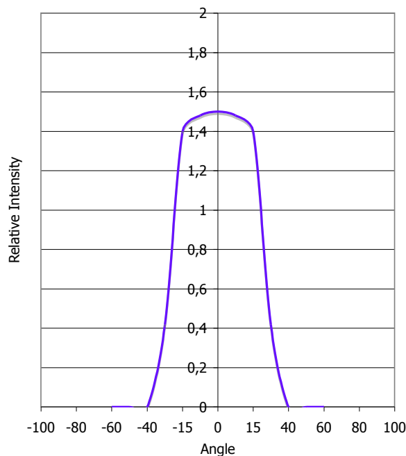
Spectrum Distribution
