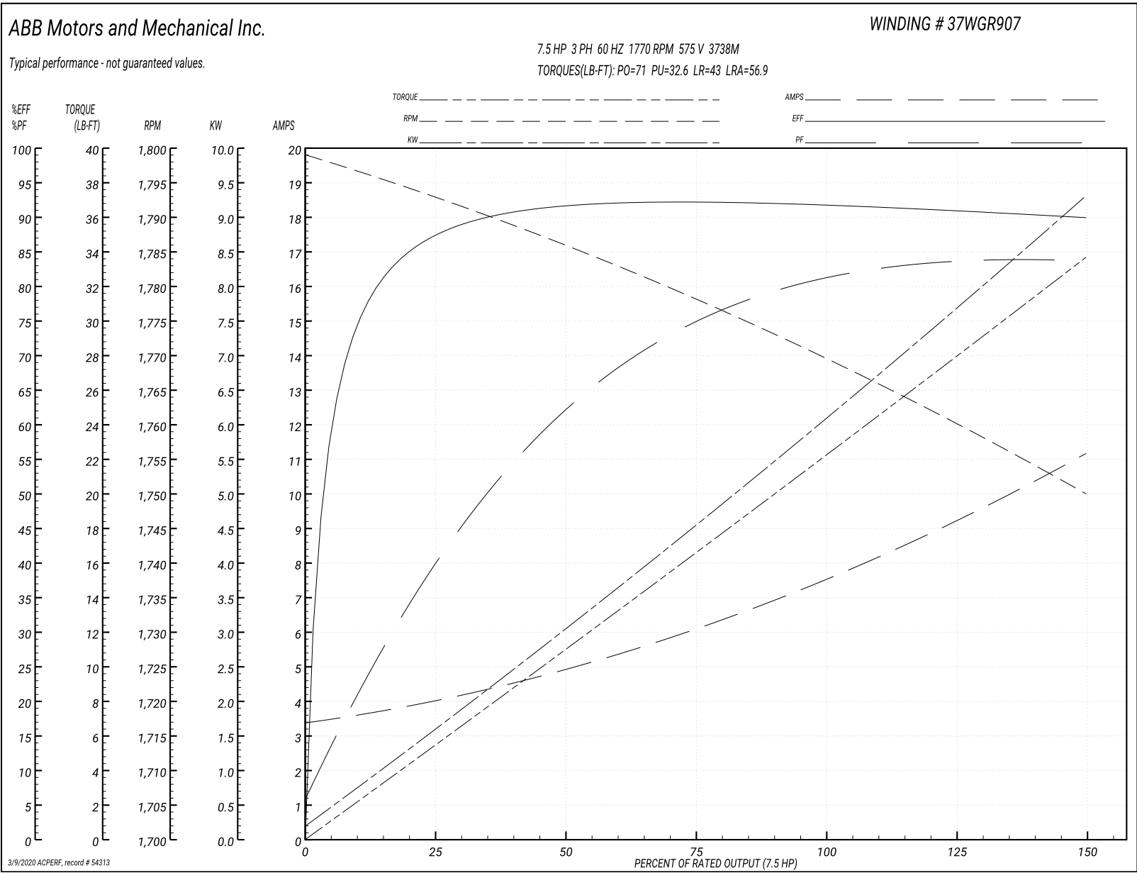
Performance Graph at 575V, 60Hz, 7.5HP Typical performance - Not guaranteed values
