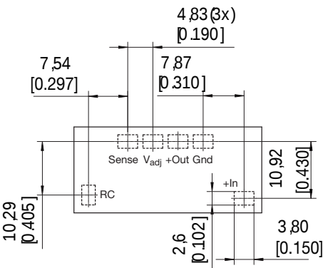
Recommended footprint. Top View
