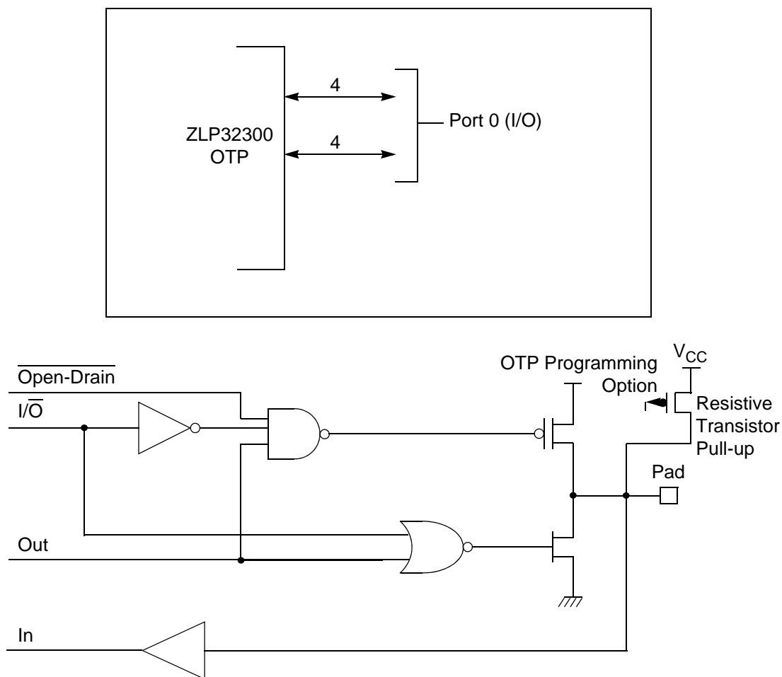
Figure 7. Port 0 Configuration
