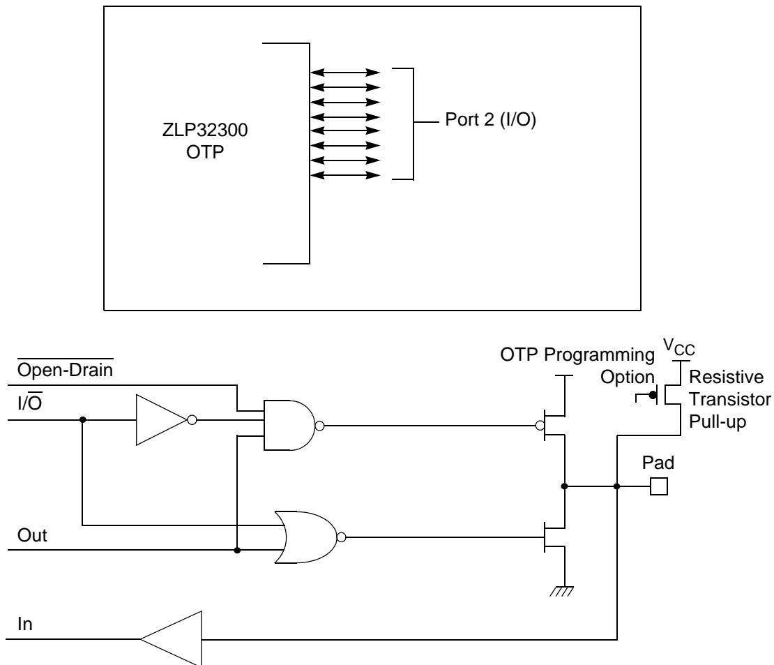
Figure 9. Port 2 Configuration
