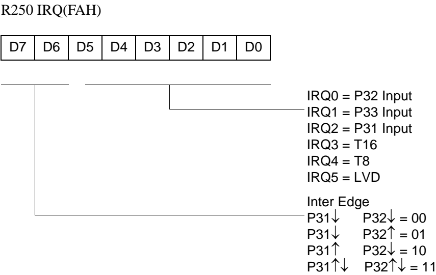
Figure 50. Interrupt Request Register (FAH: Read/Write)
