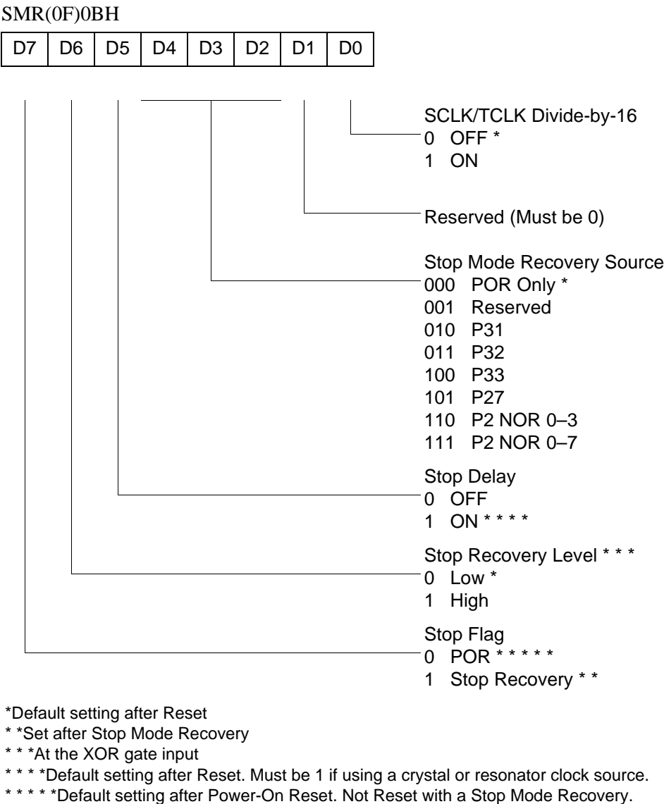
Figure 43. Stop Mode Recovery Register ((0F)0BH: D6–D0=Write Only, D7=Read Only)
