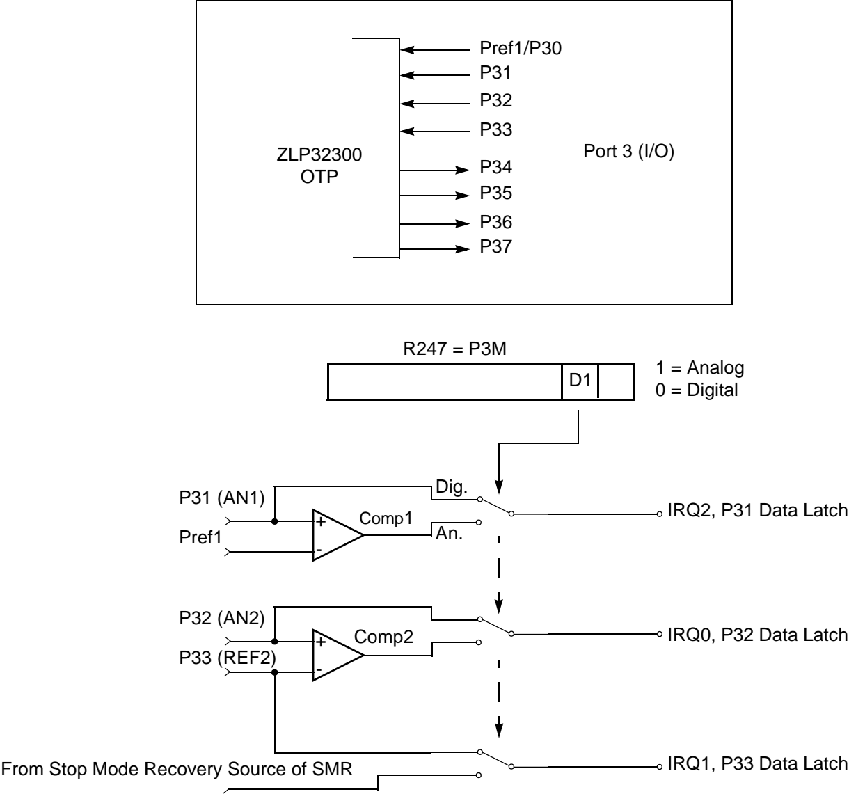
Figure 10. Port 3 Configuration
