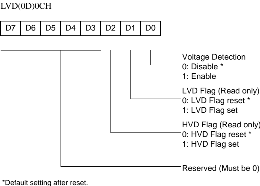
Figure 41. Voltage Detection Register
