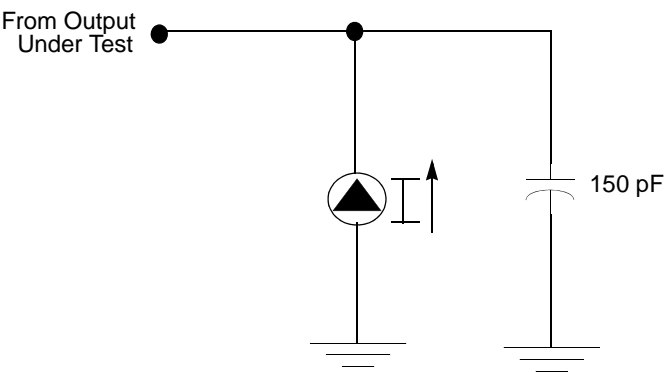
Figure 56. Test Load Diagram
