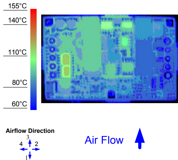
Figure 12. Thermal Image for Airflow Direction 3 (8.4A output, 55°C ambient, 200 LFM, Vin = 48V open frame unit using socket interface)
