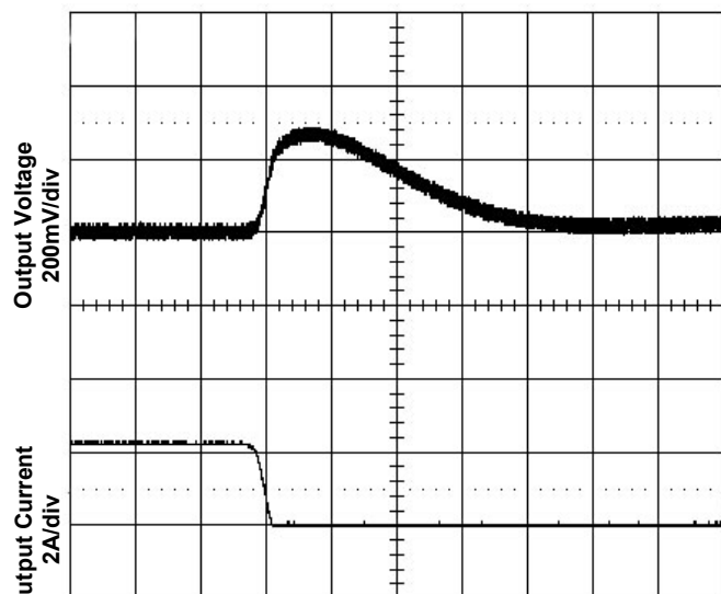
Time - t (100μs/div) Figure 7. Transient Load Response Top: Output voltage deviation Bottom: Load current step (-25% full load) Test Cond.: Output current 5A (50% full load), Input voltage 48V, Slew rate 0.1A/μs
