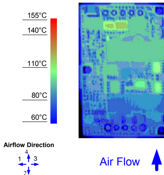
Figure 14. Thermal Image for Airflow Direction 4 (7.6A output, 55°C ambient, 200 LFM, Vin = 48V open frame unit using solder interface)
