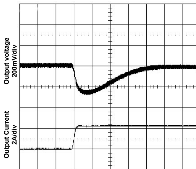
Time - t (100μs/div) Figure 8. Transient Load Response Top: Output voltage deviation Bottom: Load current step (+25% full load) Test Cond.: Output current 5A (50% full load), Input voltage 48V, Slew rate 0.1A/μs
