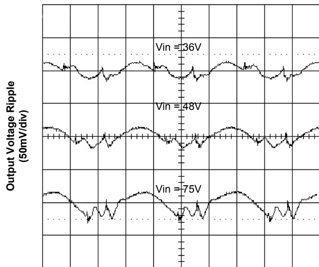
Time - t (1μs/div) Figure 5. Output Ripple Voltage at 25A Load
