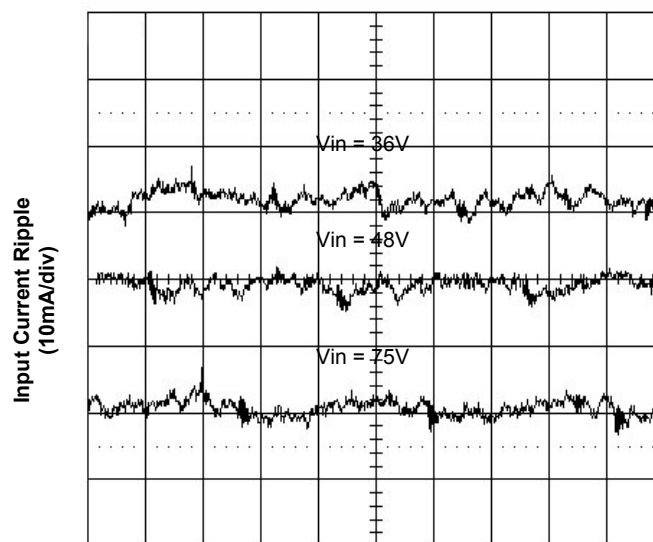
Time - t (1μs/div) Figure 6. Input Reflected Ripple Current at 25A Load
