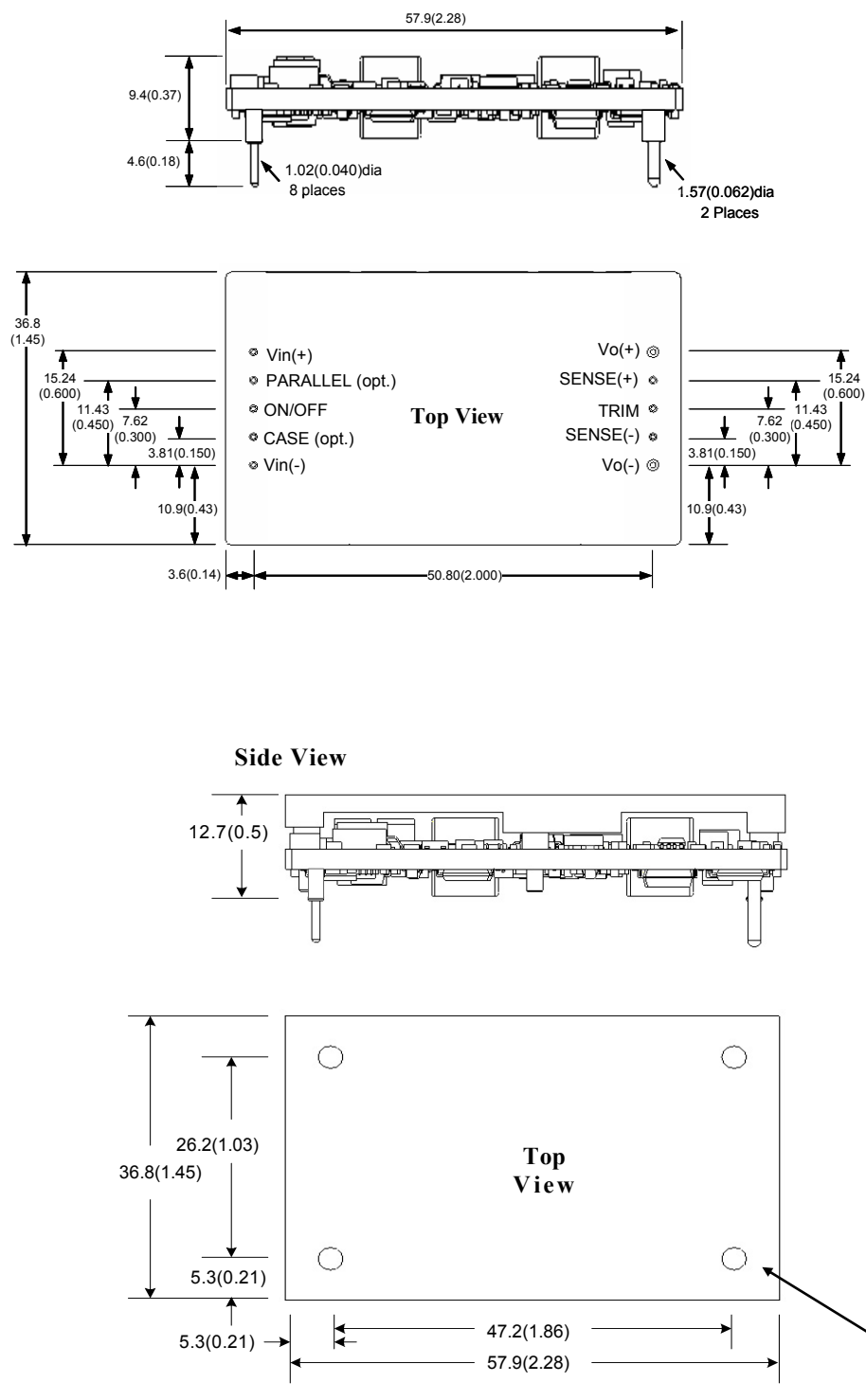
Figure 25. Converter with Optional Baseplate
