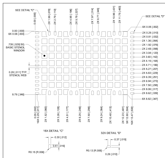
Figure 6: LGA Stencil Designs Cont'd
