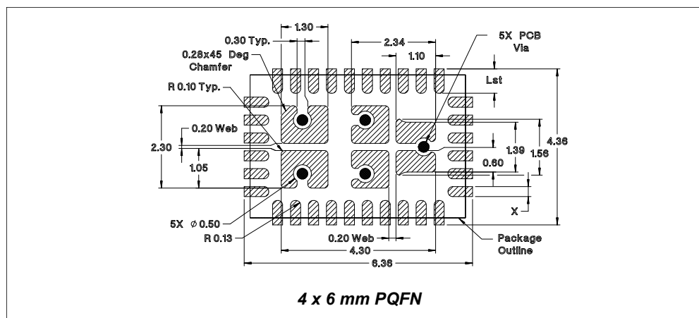
Figure 3-3 Stencil Design
