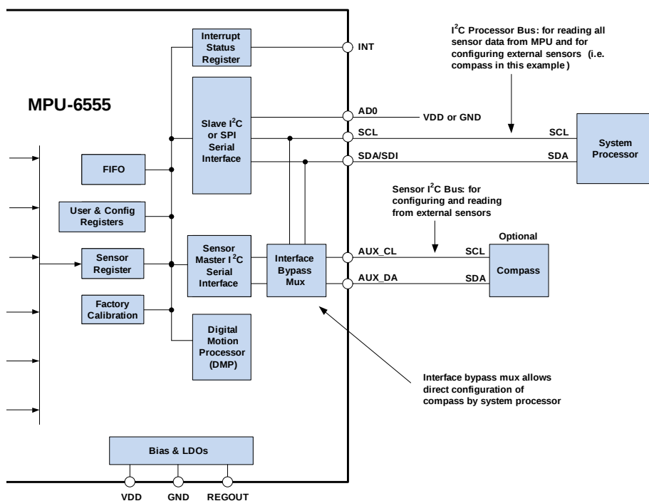
Figure 6: MPU-6555 Solution Using I 2 C Interface
