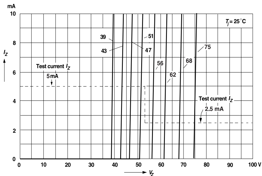
Figure 18. Breakdown Characteristics
