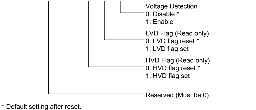
Figure 41. Voltage Detection Register
