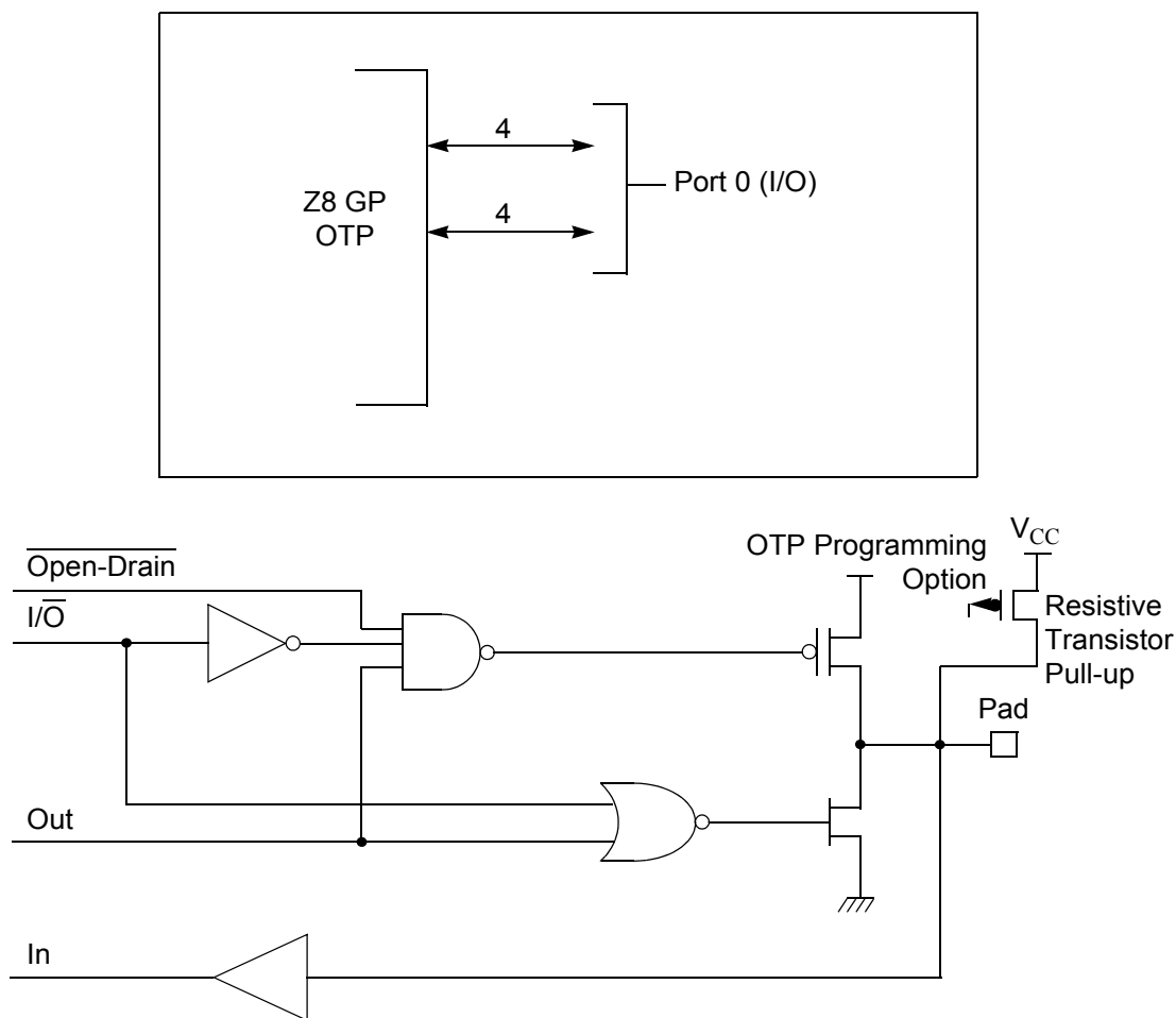
Figure 7. Port 0 Configuration
