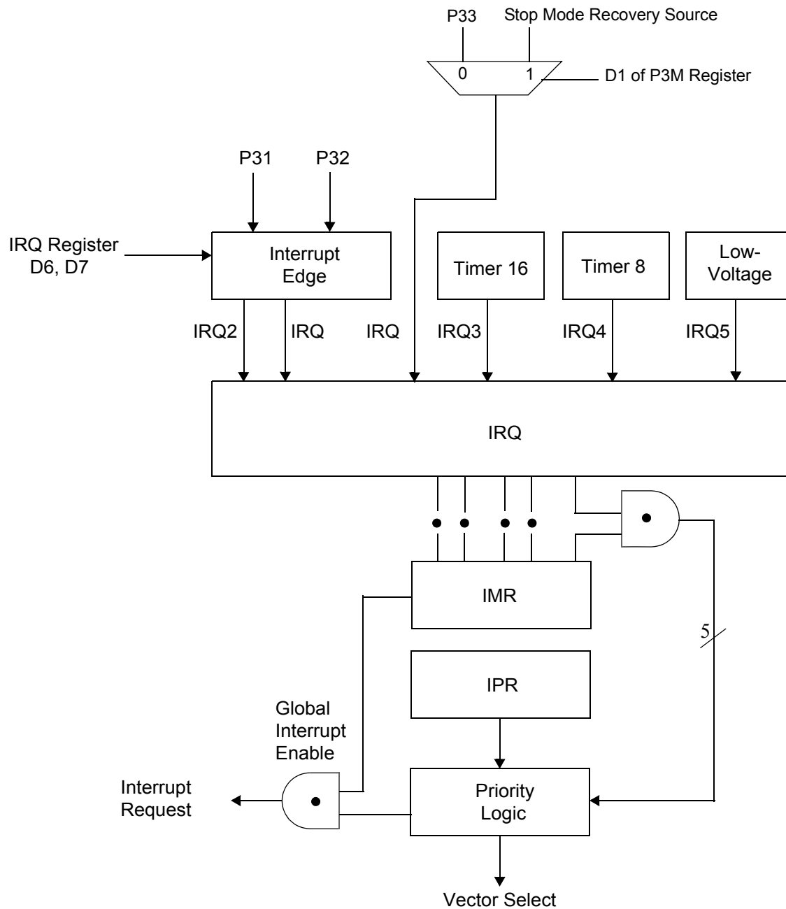
Figure 28. Interrupt Block Diagram
