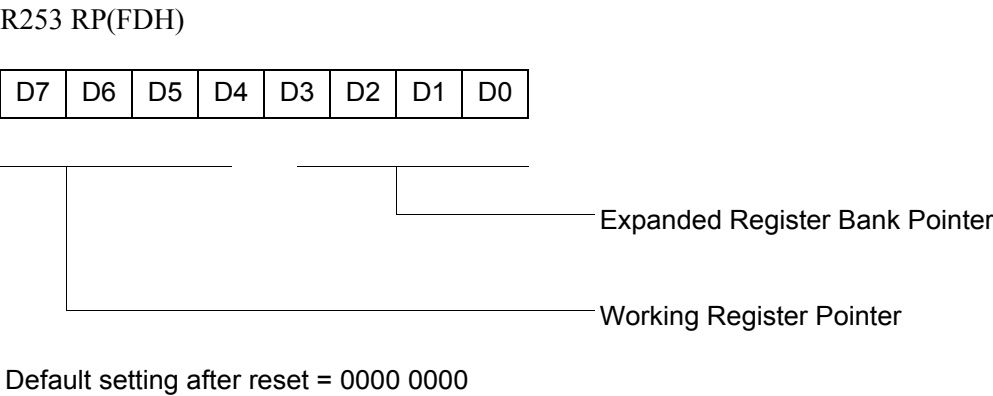
Figure 53. Register Pointer (FDH: Read/Write)
