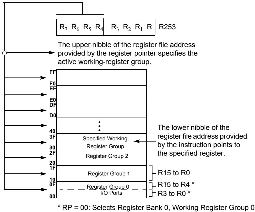
Figure 15. Register Pointer—Detail
