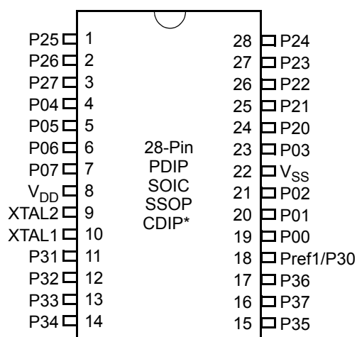
Figure 4. 28-Pin PDIP/SOIC/SSOP/CDIP* Pin Configuration
