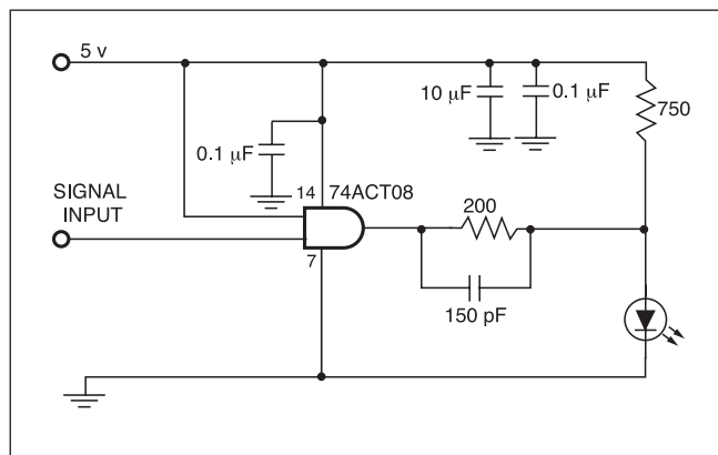
FIGURE 3. Test drive circuit ( I_F = 22\text{mA} ).
