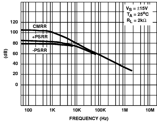
FIGURE 13. PSRR AND CMRR vs FREQUENCY
