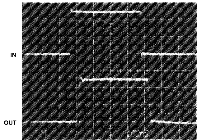
PULSE RESPONSE
