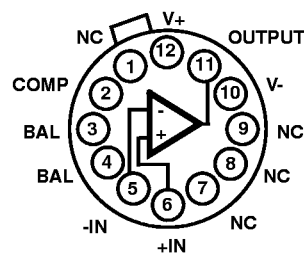
HA-2542 (METAL CAN) TOP VIEW
