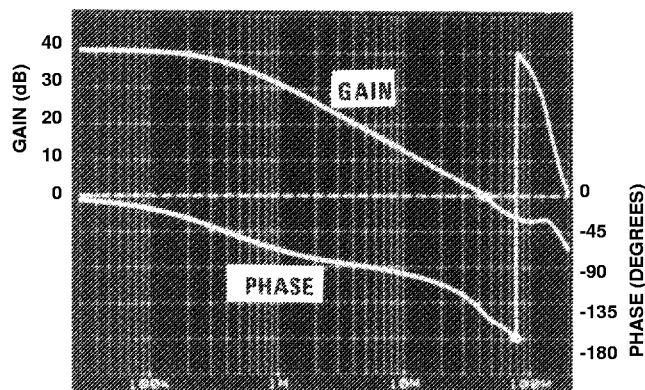
FREQUENCY RESPONSE
