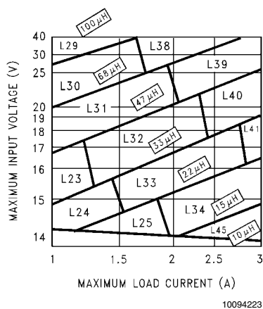
FIGURE 5. LM2670-12
