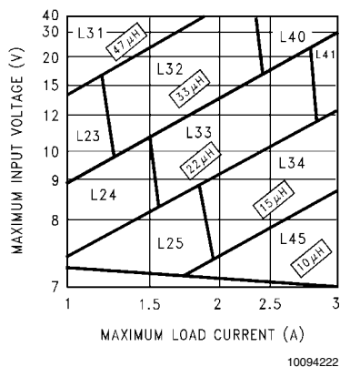
FIGURE 4. LM2670-5.0
