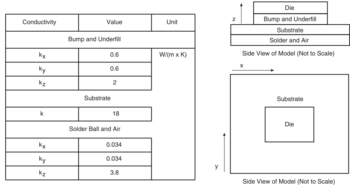
Figure 6-5. Recommended Thermal Model of PC7447 and PC7457
