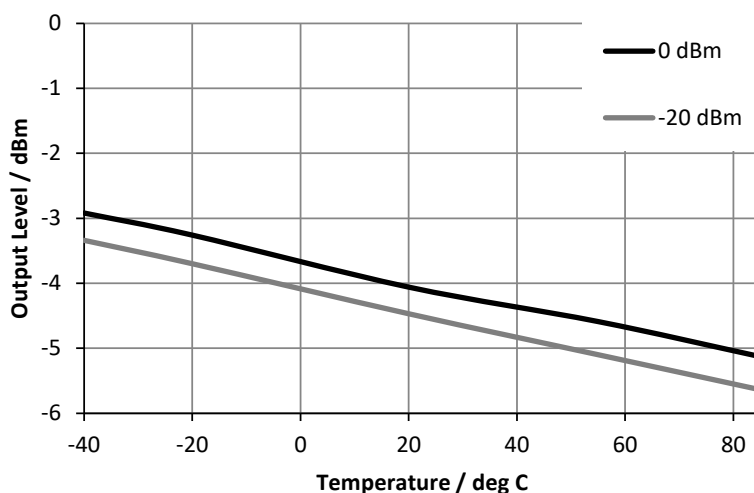
Figure 32 Typical Tx Output Level (No Divider) vs. Temperature for Varying LO Input Level
