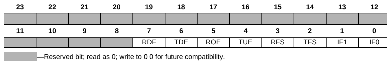
Figure 7-11. ESSI Status Register (SSISR)
