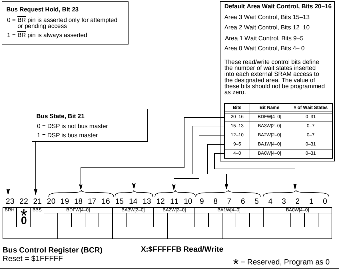
Figure B-5. Bus Control Register (BCR)
