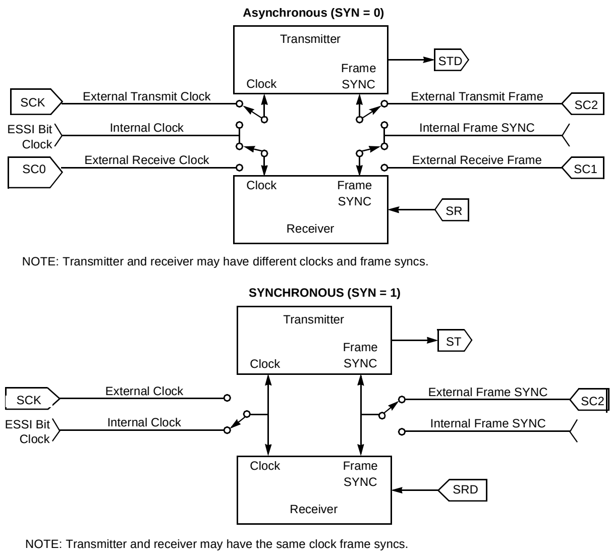
Figure 7-7. CRB SYN Bit Operation
