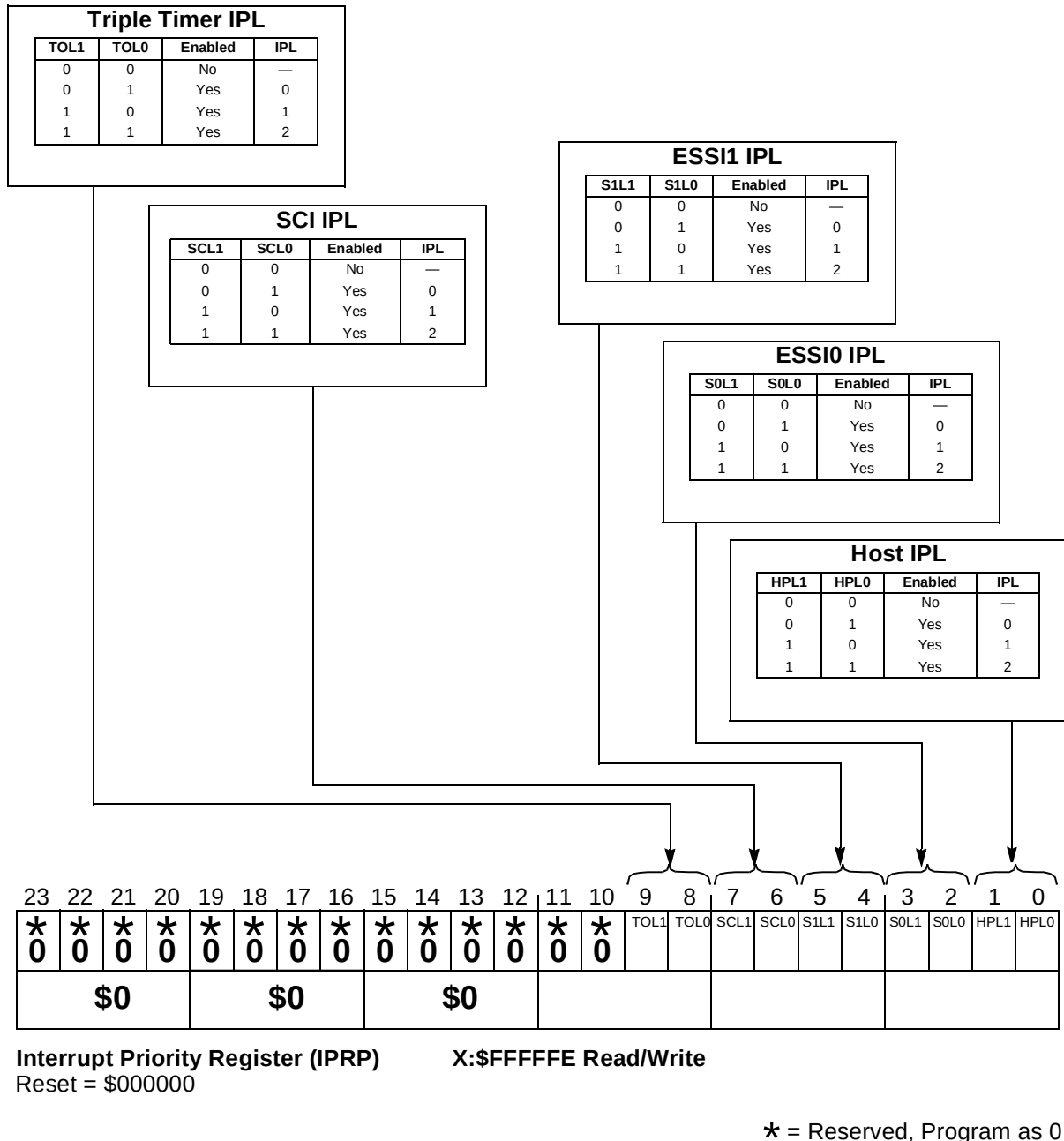
Figure B-3. Interrupt Priority Register-Peripherals (IPRP)
