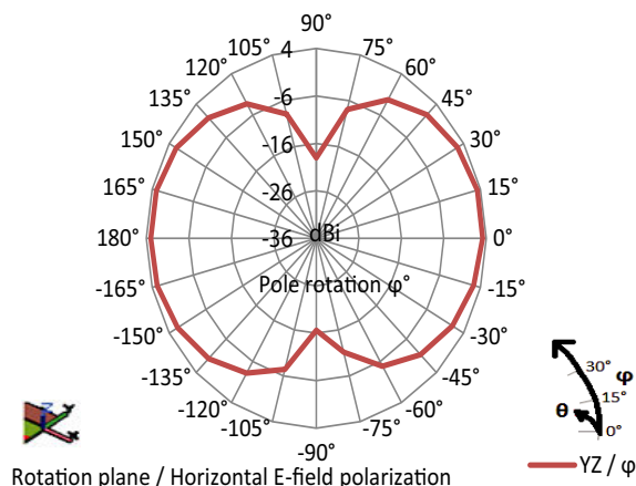
Fig. 5 - VJ5601M868MXBSR YZ Radiation Pattern
