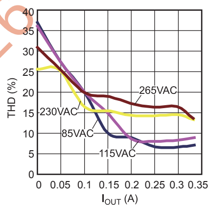
THD vs. I_{OUT}
