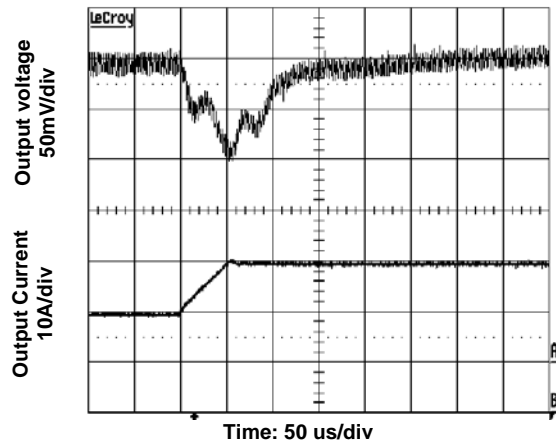
Figure 9. Transient Load Response. Output current 10A (50% full load), Input voltage 5V, Slew rate 0.2A/µs.
