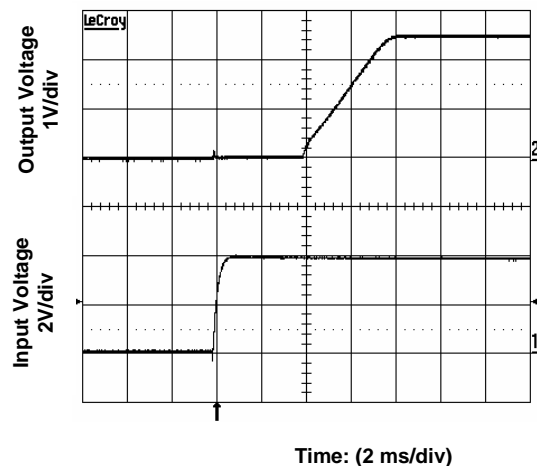
Figure 5. Start-Up from Application of Input Voltage Input voltage 4V, Output current 20A
