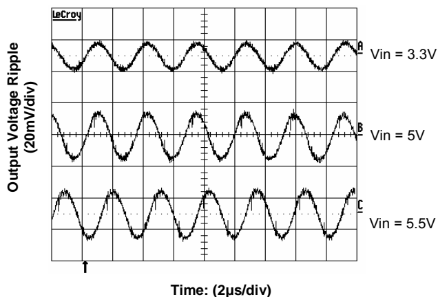
Figure 4. Output Ripple Voltage at 2.5V, 20A Output
