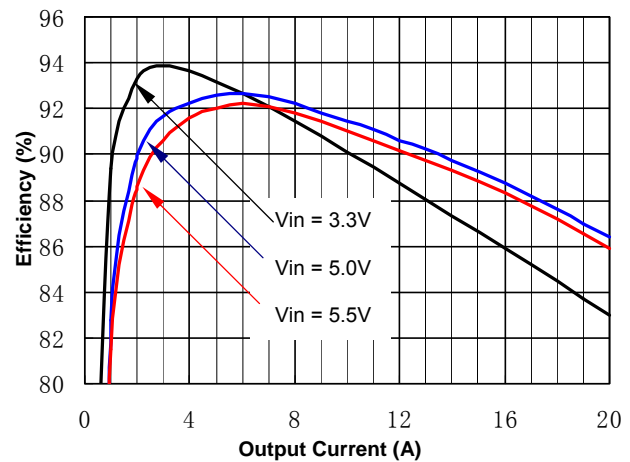
Figure 1(b). Efficiency vs. Load Current (25°C, 1.0V output)
