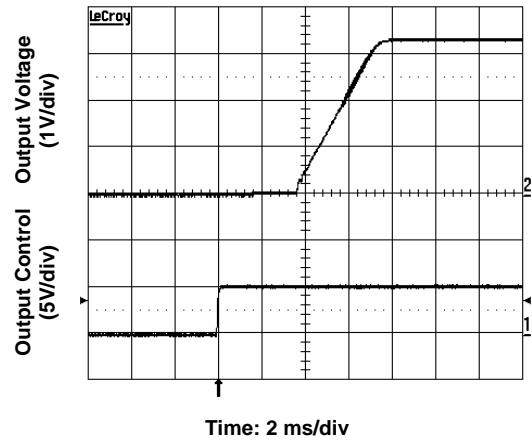
Figure 3. Start-Up from Enable Control Input voltage 5V, Output current 20A
