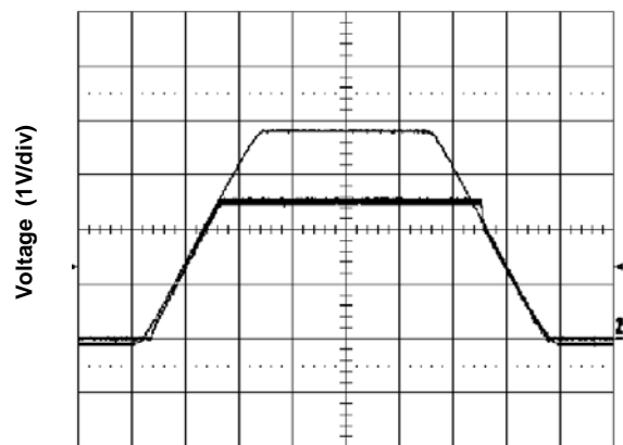
Figure 11 Voltage Tracking/Sequencing (with tracking option) Vin = 4V, Vo = 2.5V, Io = 0A
