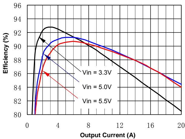
Figure 1(a). Efficiency vs. Load Current (25°C, 0.8V output)
