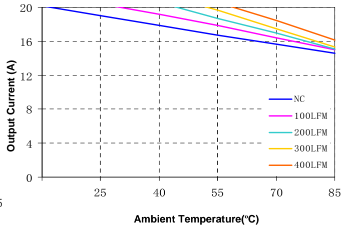
Figure 12(f). Current Derating Curve for 3.3V Output (Vin = 5V open frame)
