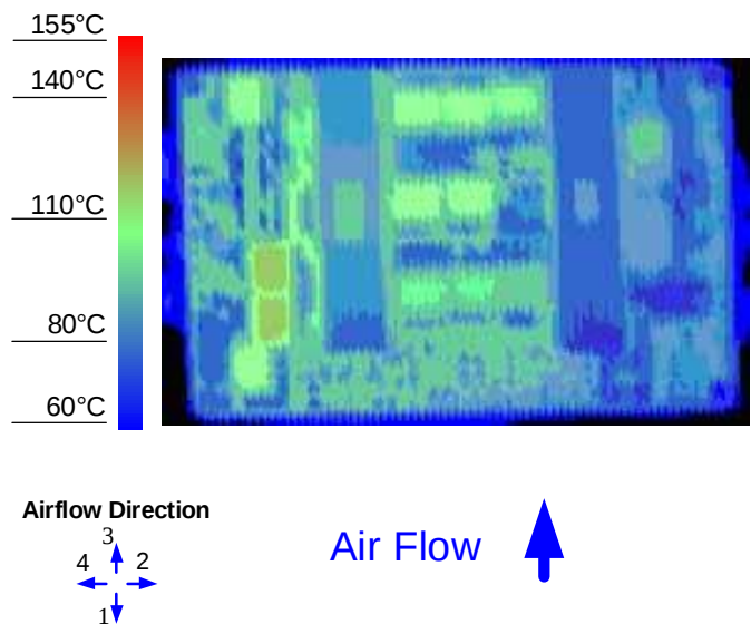
Figure 12. Thermal Image for Airflow Direction 3 (41.5A output, 55 ^{\circ}C ambient, 200 LFM, V_{in} = 48V open frame unit using socket interface)
