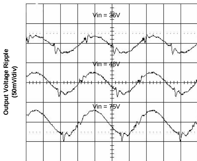
Time - t (1 \mu s/div) Figure 5. Output Ripple Voltage at 60A Load
