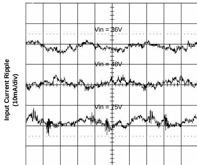
Time - t (1 \mu s/div) Figure 6. Input Reflected Ripple Current at 60A Load
