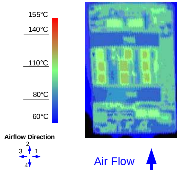
Figure 14. Thermal Image for Airflow Direction 2 (39A output, 55°C ambient, 200 LFM, Vin = 48V open frame unit using solder interface)
