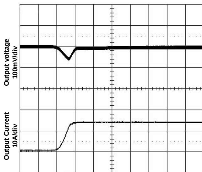
Time - t (200 \mu s/div) Figure 8. Transient Load Response
