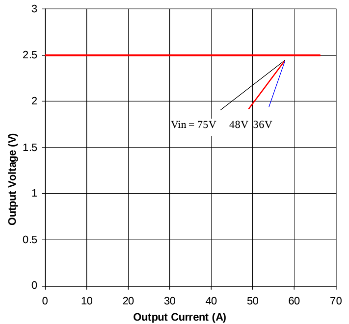
Figure 10. Output Characteristics
