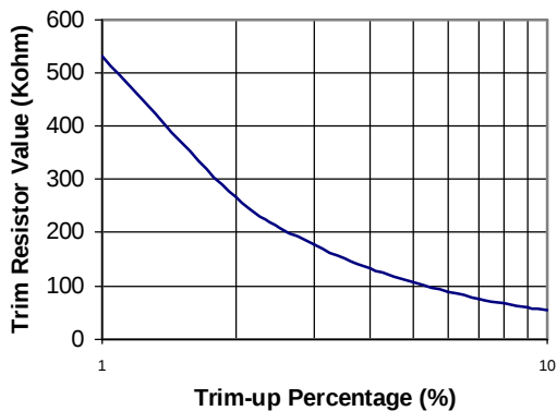
Fig. 19 Trim-Up Resistor Selection
