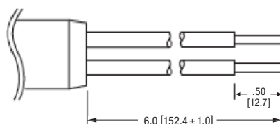
6" Wire Leads
