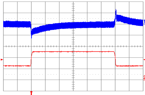
Fig. 5.0V.11: Output voltage response to load current step-change (2.5A – 5A – 2.5A) at V_{in} = 24V . Top trace: output voltage (100 mV/div.). Bottom trace: load current (2 A/div.). Current slew rate: 0.1 A/ \mu s . C_o = 1 \mu F ceramic. Time scale: 0.2 ms/div.
