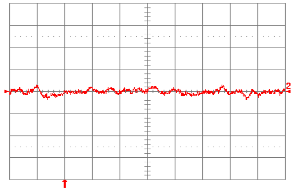
Fig. 1.8V.16: Input reflected ripple current, i_s (10 mA/div.), measured through 10 \mu\text{H} at the source at full rated load current and V_{in} = 24\text{V} . Refer to Fig. 1.8V.14 for test setup. Time scale: 1 \mu\text{s}/\text{div} .
