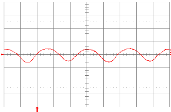
Fig. 1.8V.15: Input reflected ripple current, i_c (100 mA/div.), measured at input terminals at full rated load current and V_{in} = 24\text{V} . Refer to Fig. 1.8V.14 for test setup. Time scale: 1 \mu\text{s}/\text{div} .
