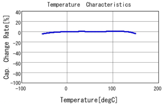
■ GCJ188R92A473KA01 C-Temp. capchange, DC0.0V, AC1.0Vrm
