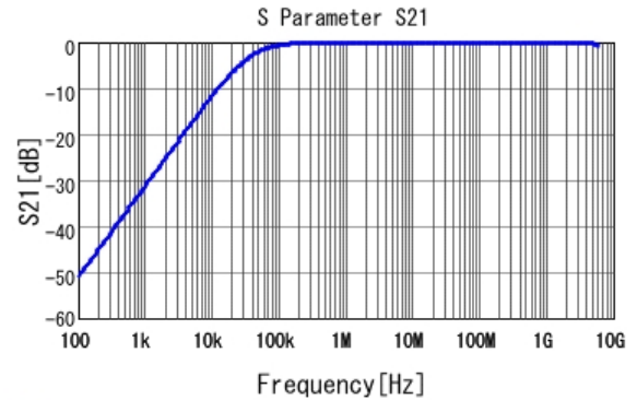
■ GCJ188R92A473KA01 S21 DC0V, 25degC
