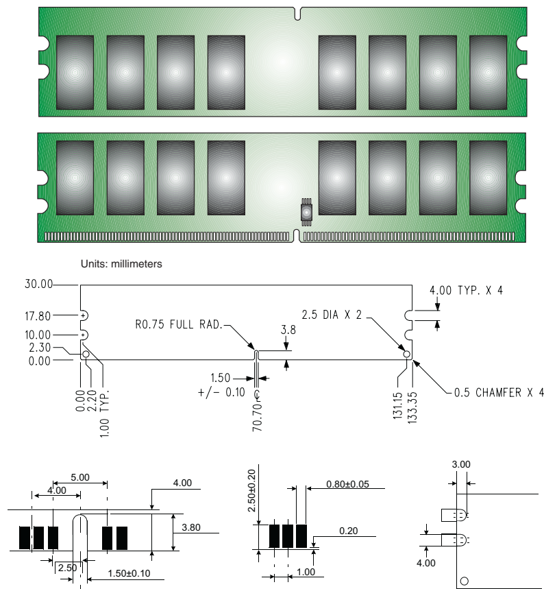
Figure 1: KVR800D2N6/1G 240-Pin DIMM
