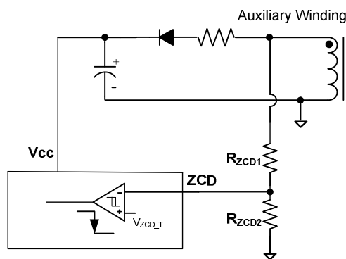
Figure 3: Zero-Current Detector
