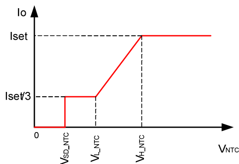
Figure 19: NTC Curve
