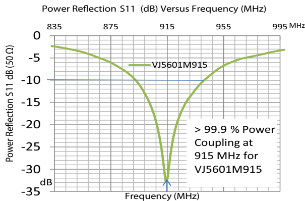
Fig. 2 - VJ5601M915 Tuned to 915 MHz with > 99.9 % Power Coupled
