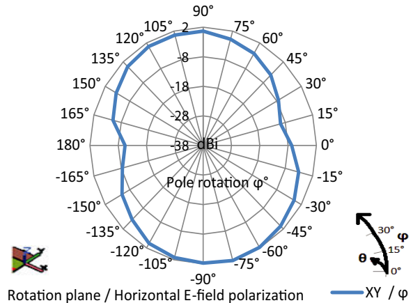
Fig. 4 - VJ5601M915MXBSR XY Radiation Pattern
