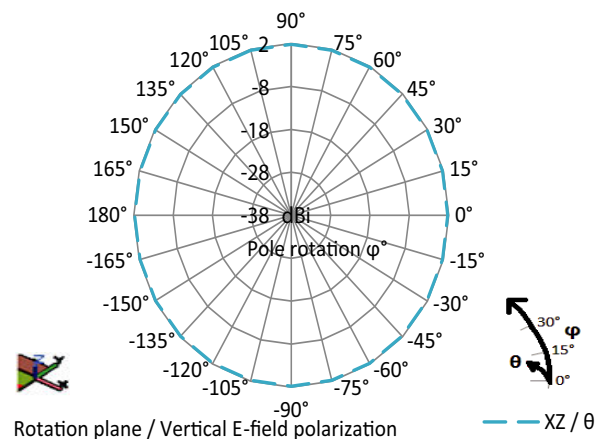
Fig. 6 - VJ5601M915MXBSR XZ Radiation Pattern
