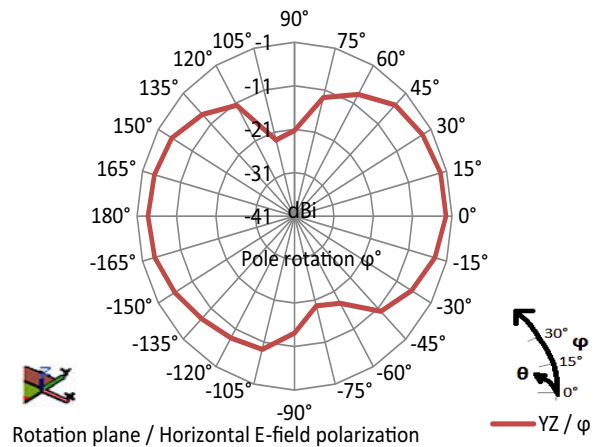
Fig. 5 - VJ5601M915MXBSR YZ Radiation Pattern
