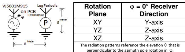
Fig. 3 - VJ5601M915 PCB Mounting and Coordinate Directions
