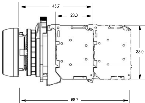
Back-of-Panel Components — Contact Cartridges with Latch
