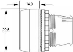
Non-Illuminated Guarded, Illuminated and Non-Illuminated Alternate Action Push Button Operators
