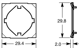
Anti-Rotation Washer
