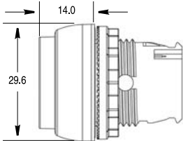
Illuminated and Non-Illuminated Momentary Extended Push Button Operators
