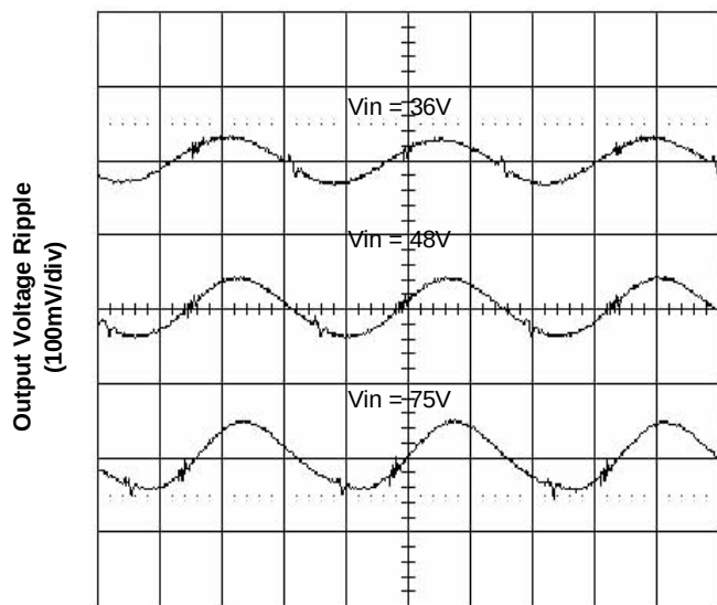
Figure 5. Output Ripple Voltage at 40A Load
