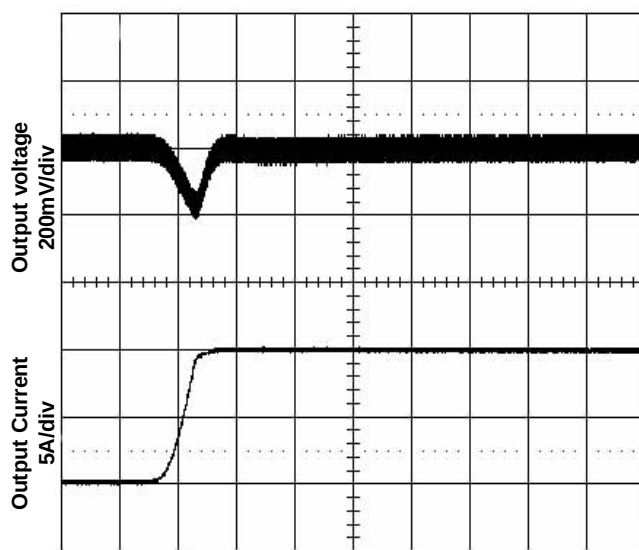
Figure 8. Transient Load Response
