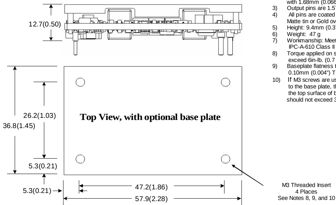
Figure 24. Converter with Optional Baseplate
