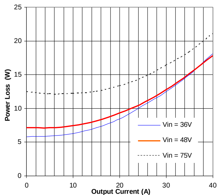
Figure 2. Power Loss vs. Load Current (25°C)
