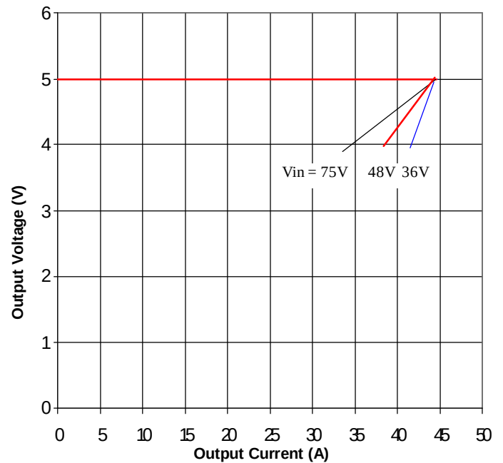
Figure 10. Output Characteristics
