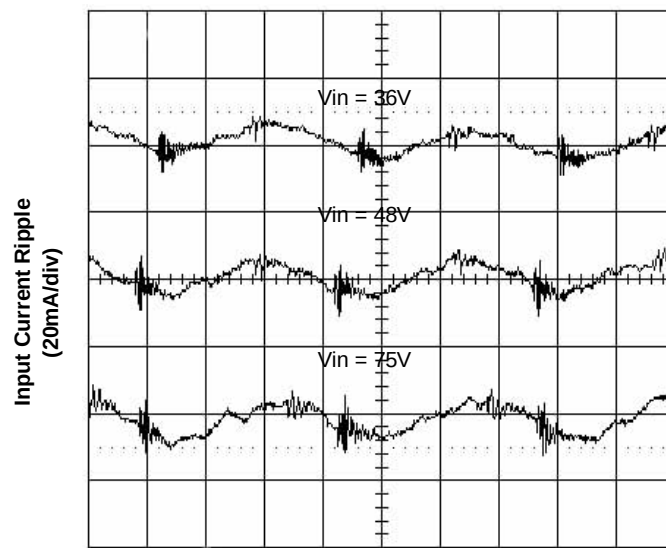
Figure 6. Input Reflected Ripple Current at 40A Load
