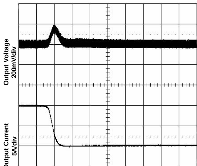
Figure 7. Transient Load Response
