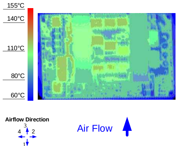
Figure 12. Thermal Image for Airflow Direction 3 (27A output, 55°C ambient, 200 LFM, Vin = 48V open frame unit using socket interface)
