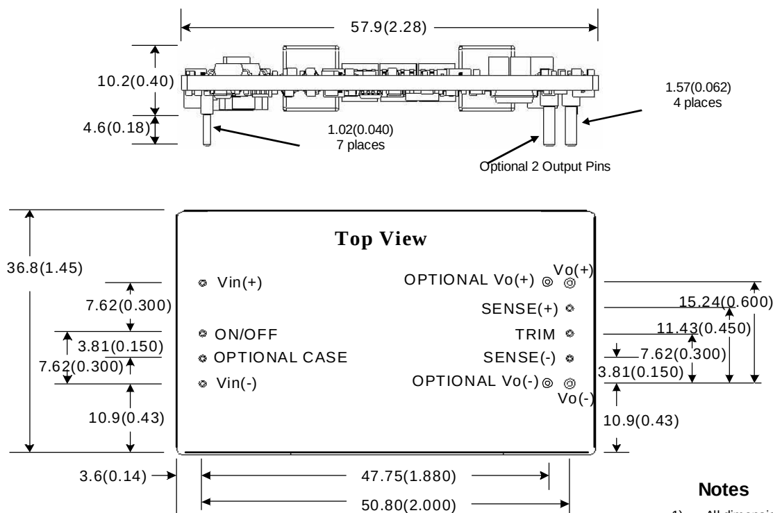
Figure 23. Open frame converter
