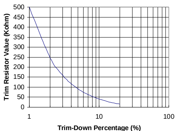
Fig. 18 Trim-Down Resistor Selection
