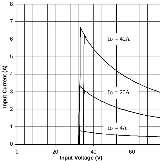
Figure 9. Input Characteristics
