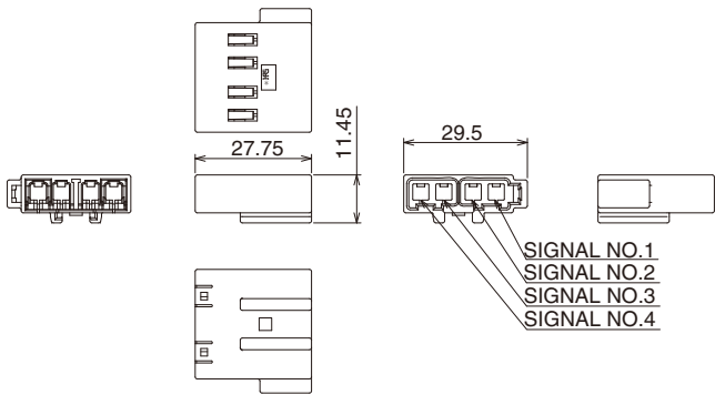
◆Retainer installed
