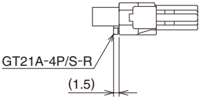
◆Retainer installed
