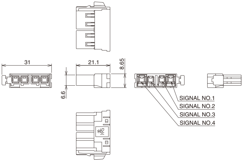
◆Retainer installed
