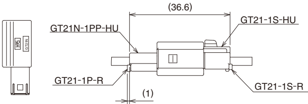
◆Mated condition
