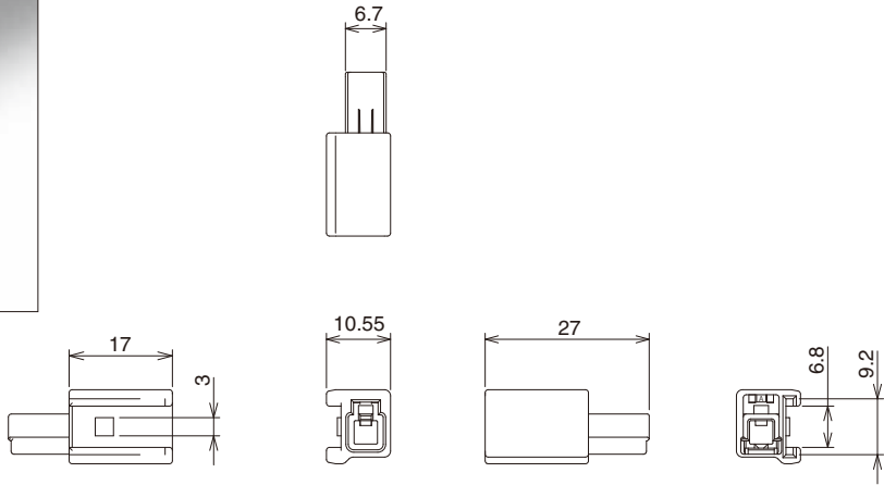
◆Mated condition
